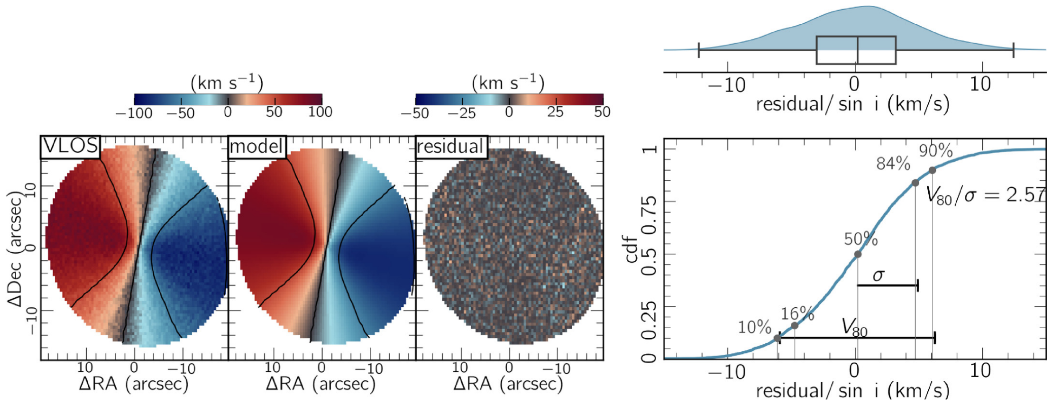
Figure 10. from Carlos López-Cobá et al 2024 Astrophys. J. 975 doi:10.3847/1538-4357/ad7b12 https://dx.doi.org/10.3847/1538-4357/ad7b12 © 2024. The Author(s). Published by the American Astronomical Society.
