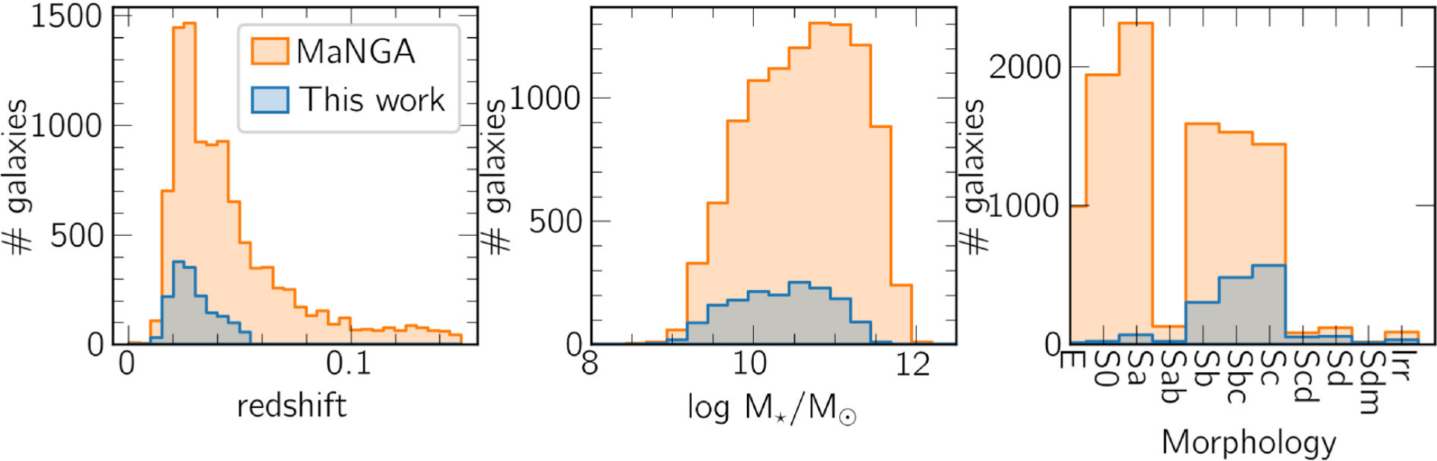
Figure 1. from Carlos López-Cobá et al 2024 Astrophys. J. 975 doi:10.3847/1538-4357/ad7b12 https://dx.doi.org/10.3847/1538-4357/ad7b12 © 2024. The Author(s). Published by the American Astronomical Society.
