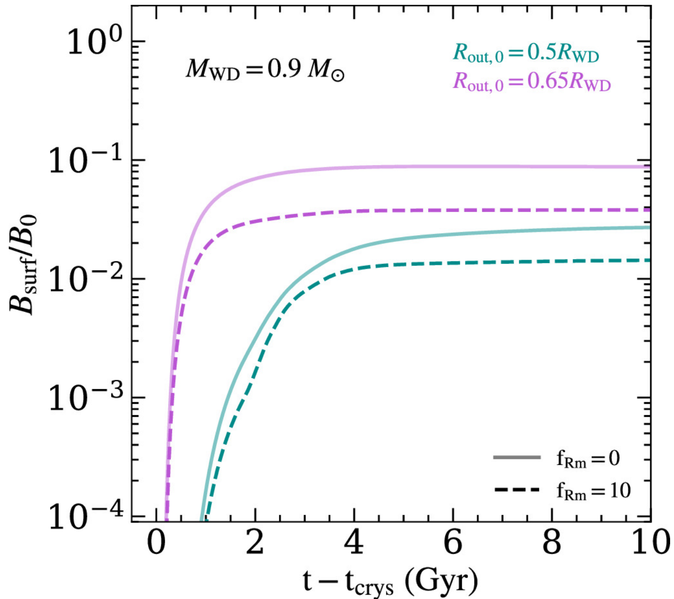
Figure 4. from Matias Castro-Tapia et al 2024 Astrophys. J. 975 doi:10.3847/1538-4357/ad7a6a https://dx.doi.org/10.3847/1538-4357/ad7a6a © 2024. The Author(s). Published by the American Astronomical Society.
