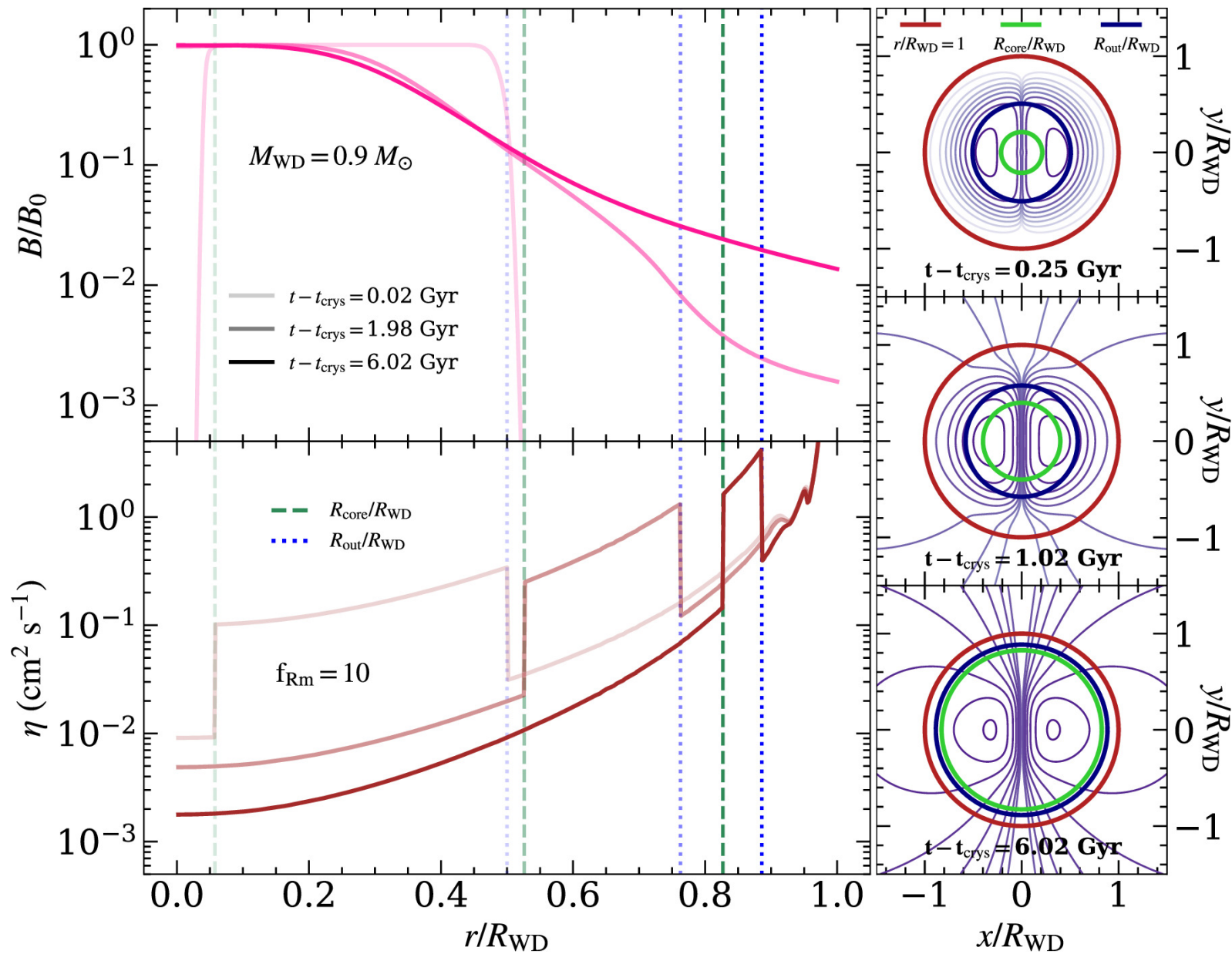
Figure 3. from Matias Castro-Tapia et al 2024 Astrophys. J. 975 doi:10.3847/1538-4357/ad7a6a https://dx.doi.org/10.3847/1538-4357/ad7a6a © 2024. The Author(s). Published by the American Astronomical Society.
