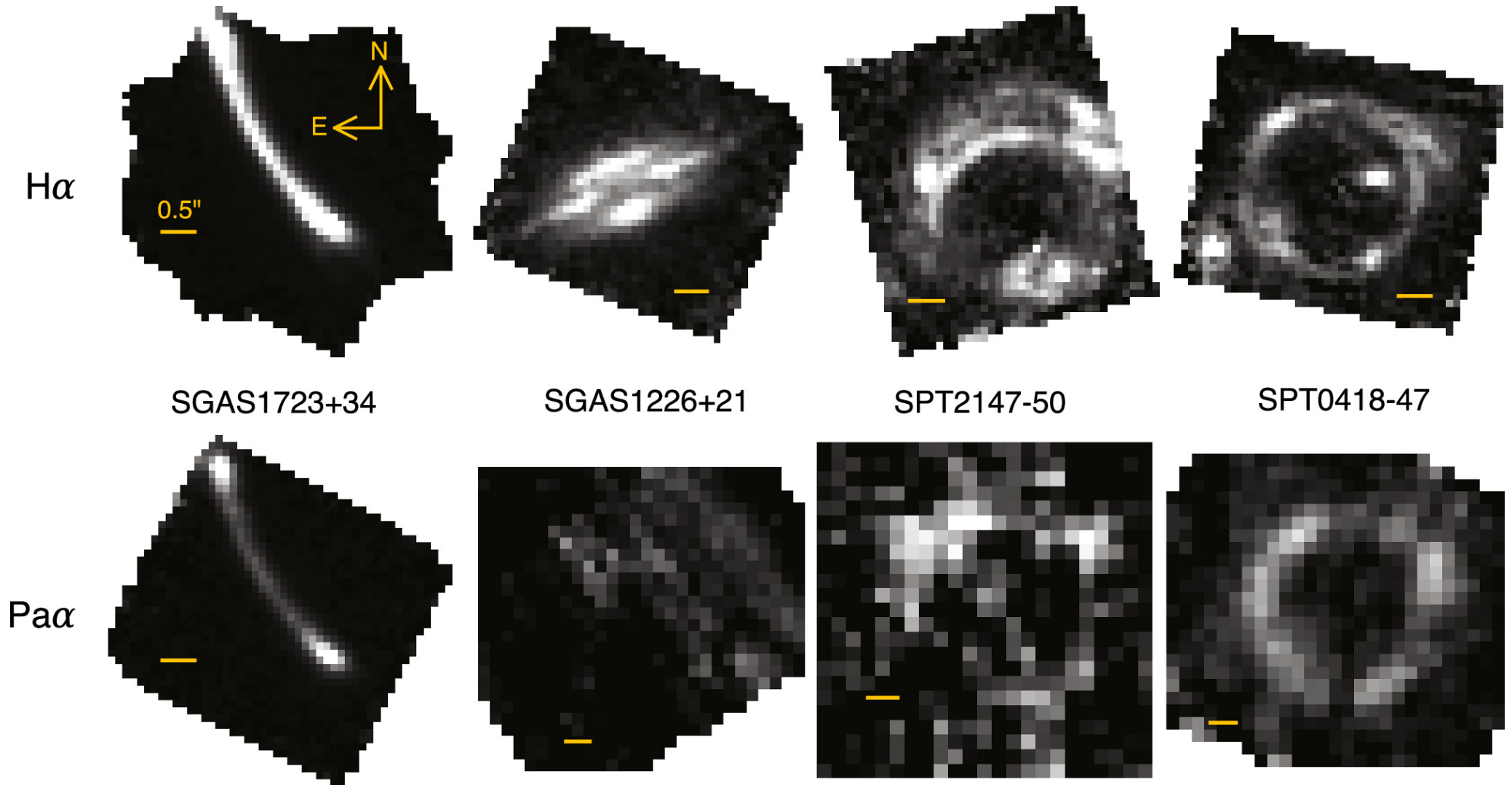
Figure 8. from Jane R. Rigby et al 2025 Astrophys. J. 978 doi:10.3847/1538-4357/ad7501 https://dx.doi.org/10.3847/1538-4357/ad7501 © 2024. The Author(s). Published by the American Astronomical Society.
