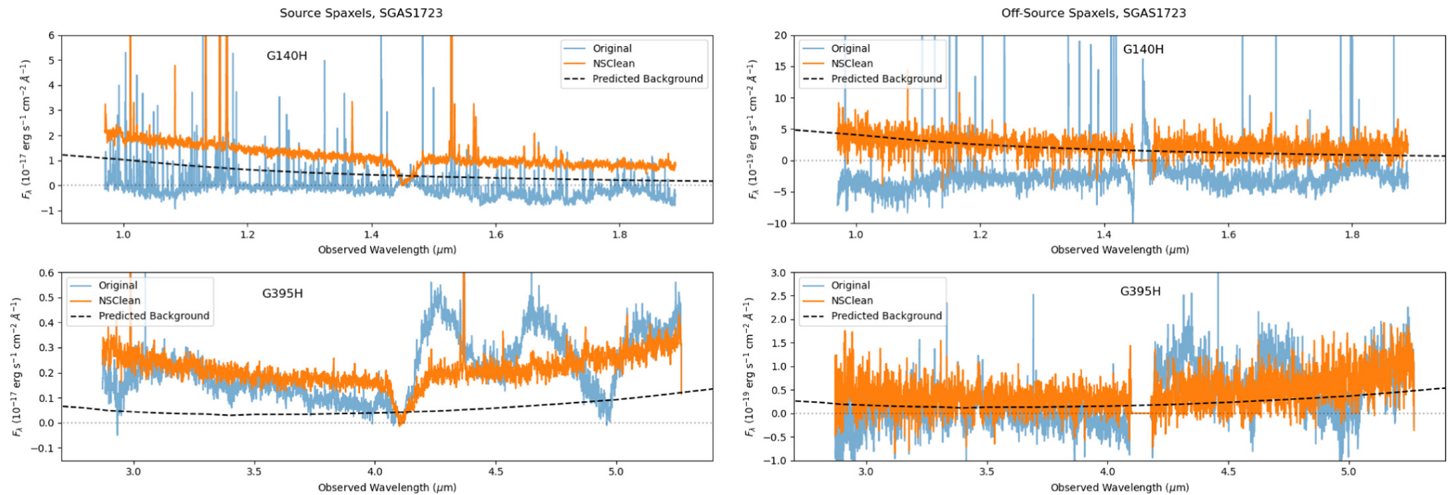
Figure 6. from Jane R. Rigby et al 2025 Astrophys. J. 978 doi:10.3847/1538-4357/ad7501 https://dx.doi.org/10.3847/1538-4357/ad7501 © 2024. The Author(s). Published by the American Astronomical Society.
