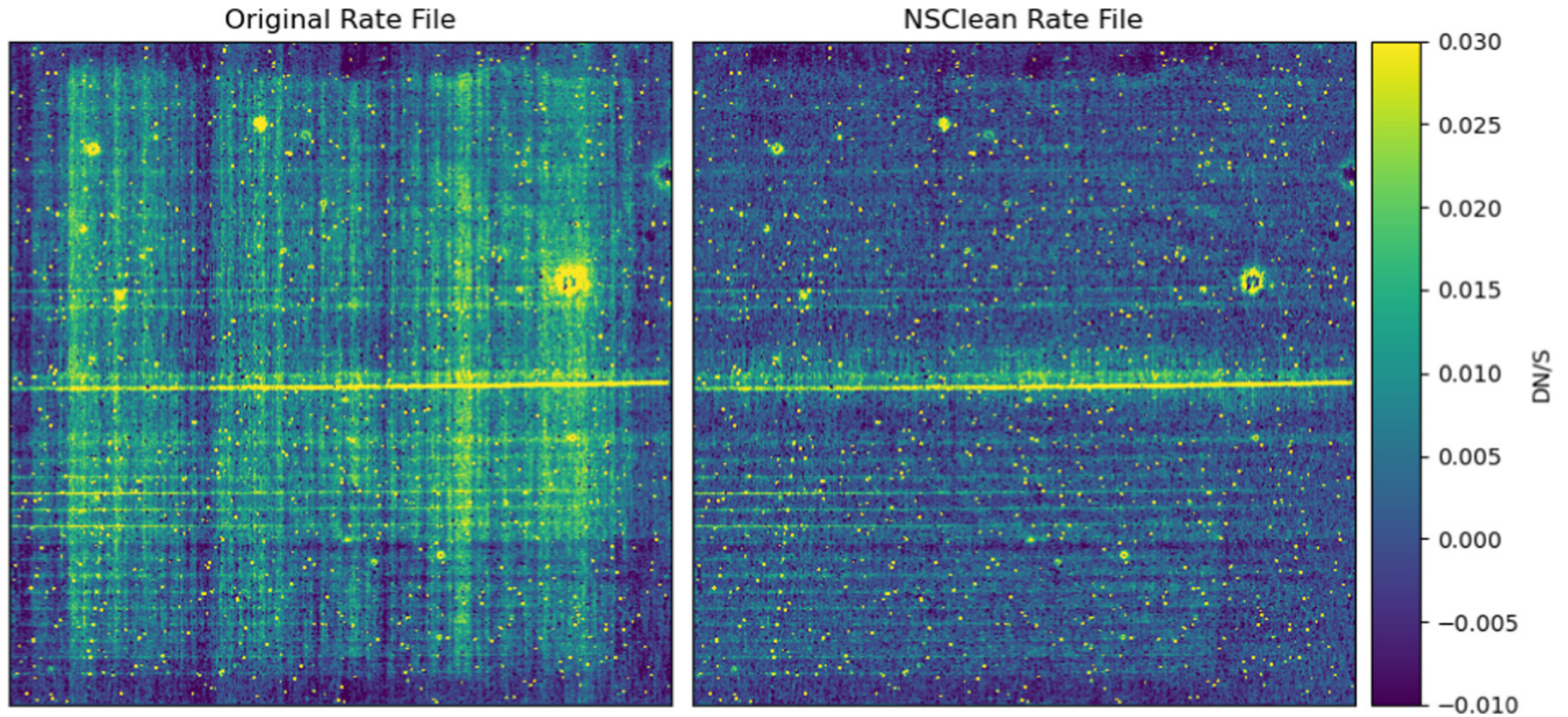
Figure 5. from Jane R. Rigby et al 2025 Astrophys. J. 978 doi:10.3847/1538-4357/ad7501 https://dx.doi.org/10.3847/1538-4357/ad7501 © 2024. The Author(s). Published by the American Astronomical Society.
