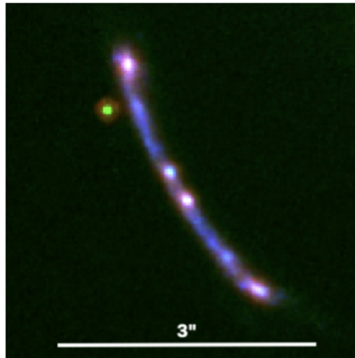
SDSS1723+34
