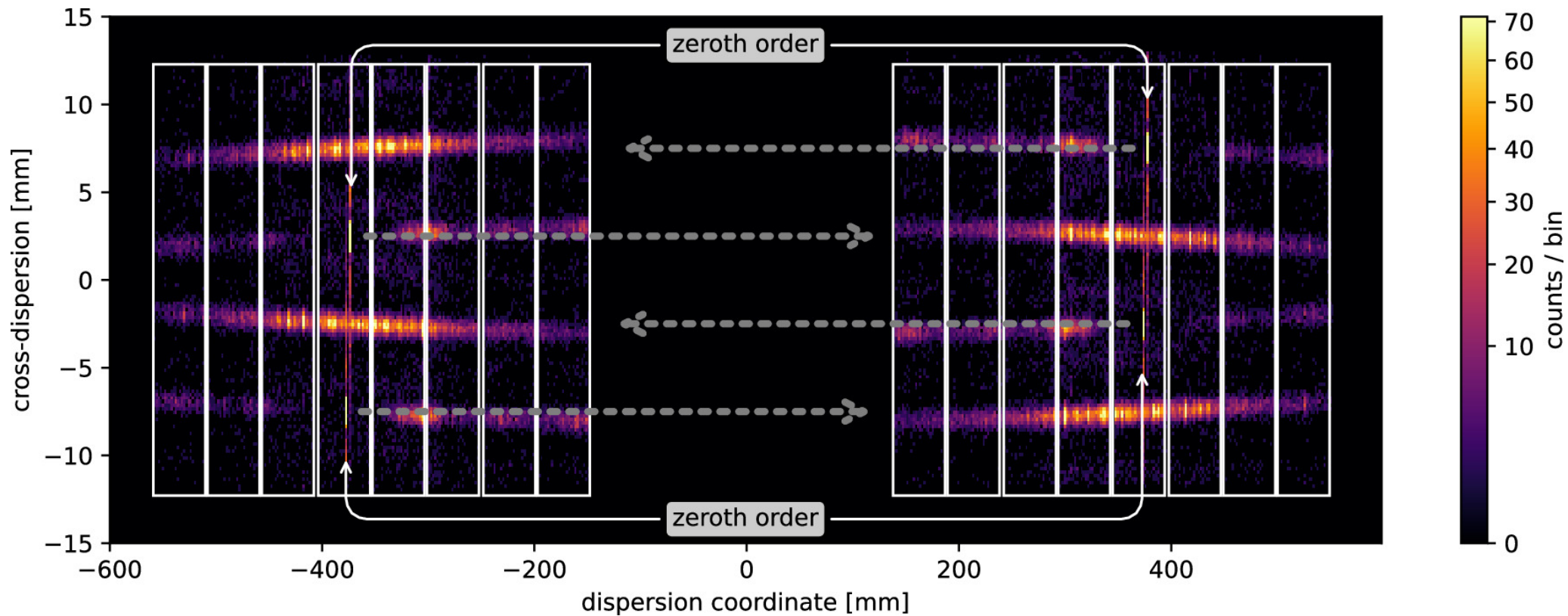
Figure 9. from Hans Moritz Günther et al 2024 Astrophys. J. 975 doi:10.3847/1538-4357/ad739c https://dx.doi.org/10.3847/1538-4357/ad739c © 2024. The Author(s). Published by the American Astronomical Society.
