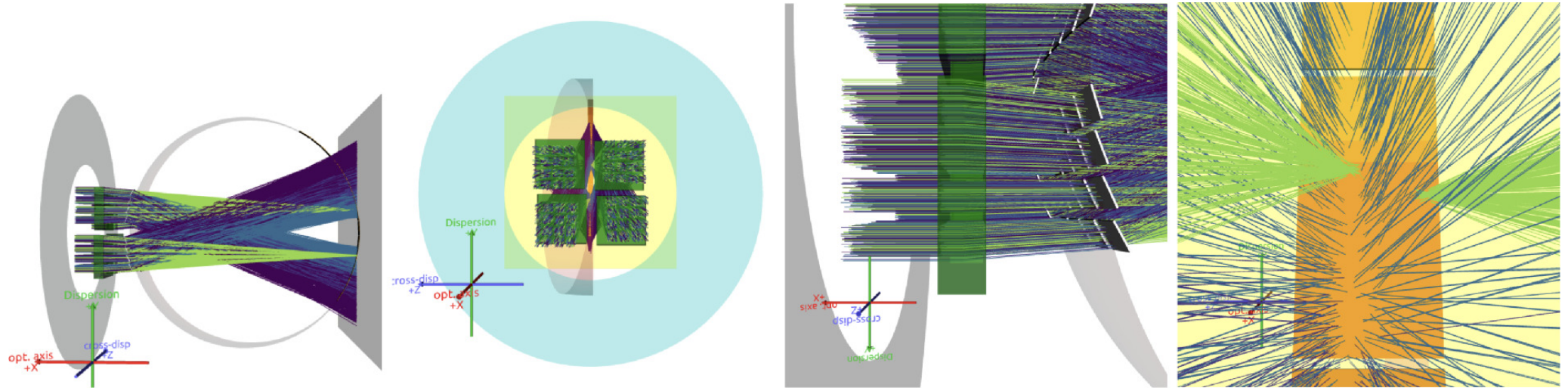
Figure 8. from Hans Moritz Günther et al 2024 Astrophys. J. 975 doi:10.3847/1538-4357/ad739c https://dx.doi.org/10.3847/1538-4357/ad739c © 2024. The Author(s). Published by the American Astronomical Society.
