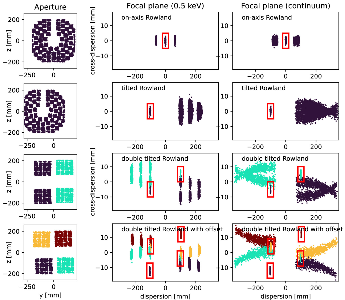
Figure 7. from Hans Moritz Günther et al 2024 Astrophys. J. 975 doi:10.3847/1538-4357/ad739c https://dx.doi.org/10.3847/1538-4357/ad739c
