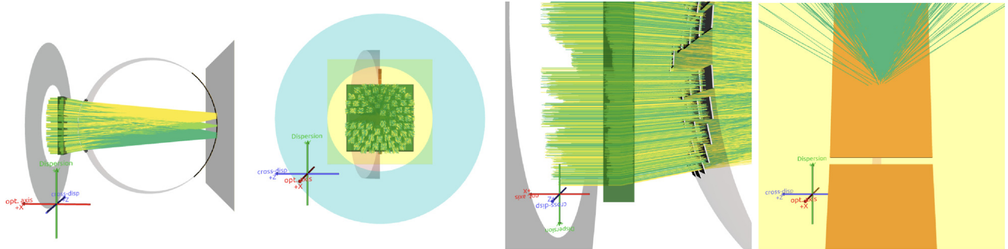
Figure 4. from Hans Moritz Günther et al 2024 Astrophys. J. 975 doi:10.3847/1538-4357/ad739c https://dx.doi.org/10.3847/1538-4357/ad739c © 2024. The Author(s). Published by the American Astronomical Society.
