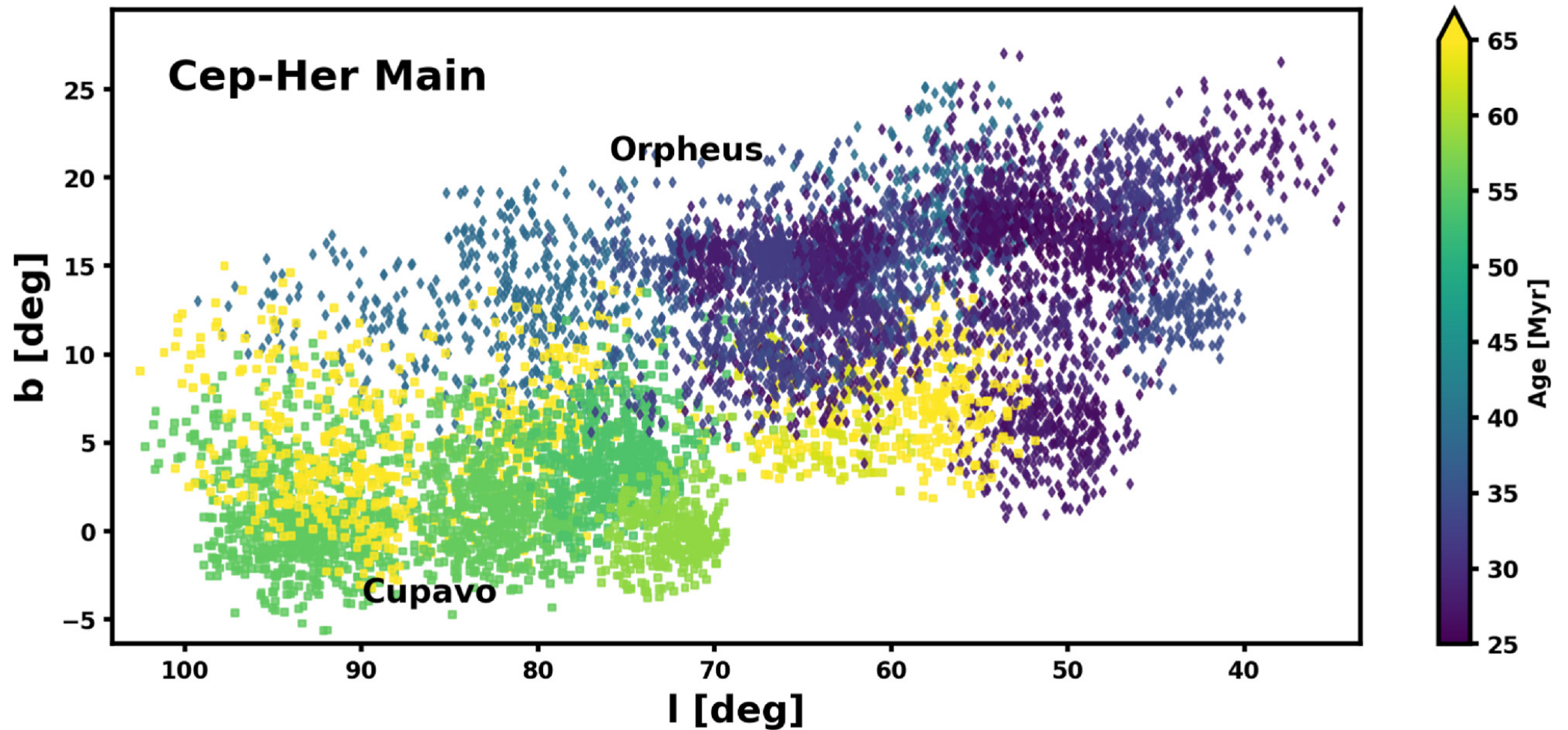
Figure 8. from Ronan Kerr et al 2024 Astrophys. J. 975 doi:10.3847/1538-4357/ad7135 https://dx.doi.org/10.3847/1538-4357/ad7135 © 2024. The Author(s). Published by the American Astronomical Society.
