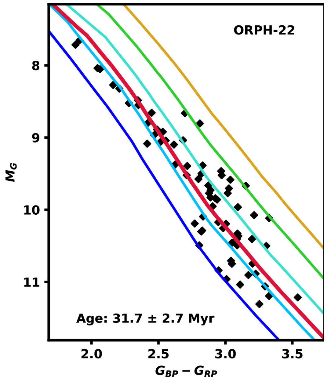
Figure 7. Age solution from Ronan Kerr et al 2024 Astrophys. J. 975 doi:10.3847/1538-4357/ad7135 https://dx.doi.org/10.3847/1538-4357/ad7135 © 2024. The Author(s). Published by the American Astronomical Society.
