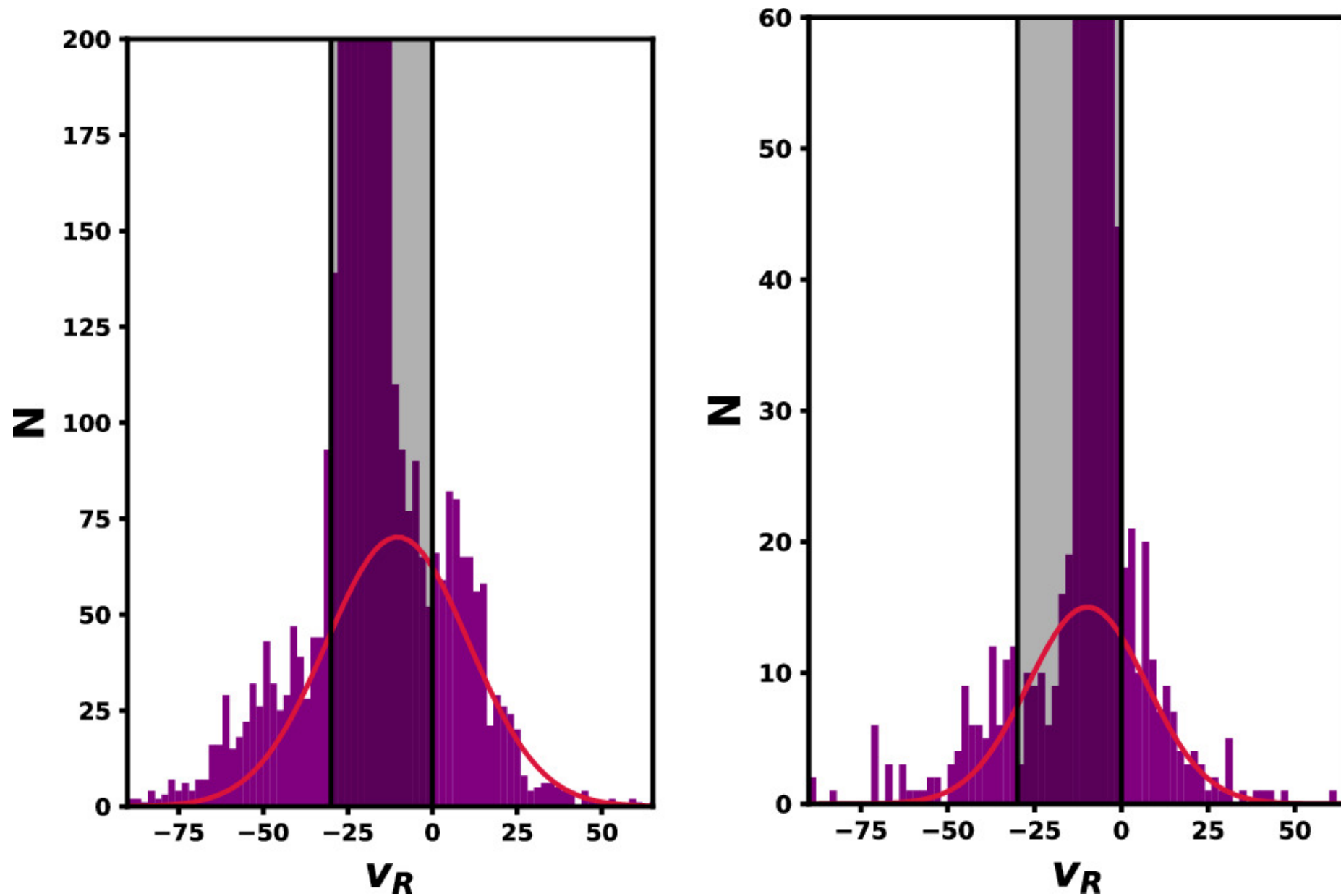
Figure 4. from Ronan Kerr et al 2024 Astrophys. J. 975 doi:10.3847/1538-4357/ad7135 https://dx.doi.org/10.3847/1538-4357/ad7135 © 2024. The Author(s). Published by the American Astronomical Society.
