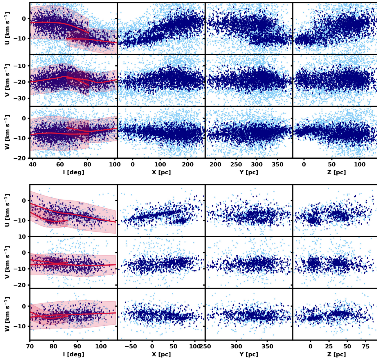
Figure 3. from Ronan Kerr et al 2024 Astrophys. J. 975 doi:10.3847/1538-4357/ad7135 https://dx.doi.org/10.3847/1538-4357/ad7135 © 2024. The Author(s). Published by the American Astronomical Society.
