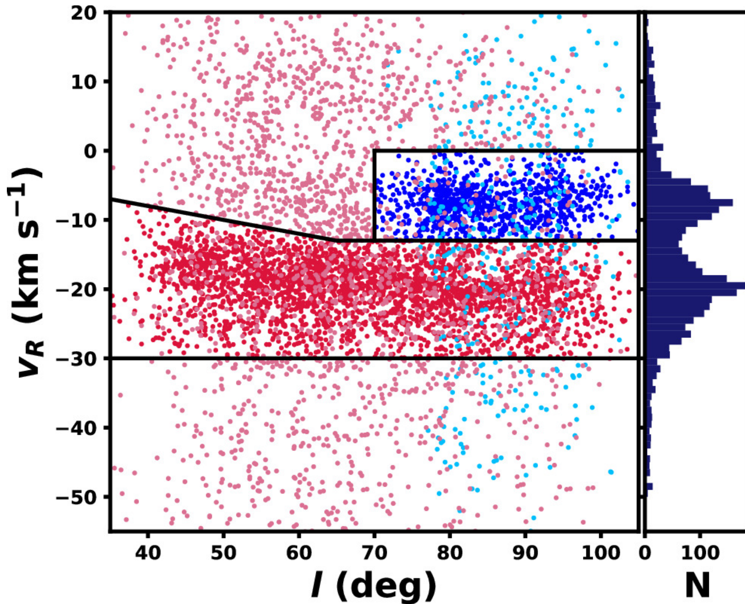
Figure 2. from Ronan Kerr et al 2024 Astrophys. J. 975 doi:10.3847/1538-4357/ad7135 https://dx.doi.org/10.3847/1538-4357/ad7135 © 2024. The Author(s). Published by the American Astronomical Society.
