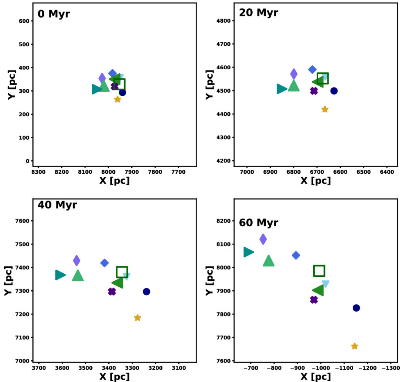
Figure 19. from Ronan Kerr et al 2024 Astrophys. J. 975 doi:10.3847/1538-4357/ad7135 https://dx.doi.org/10.3847/1538-4357/ad7135 © 2024. The Author(s). Published by the American Astronomical Society.
