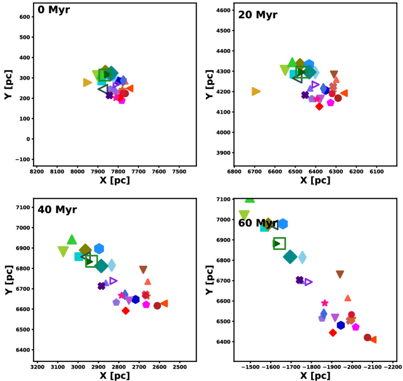
Figure 18. from Ronan Kerr et al 2024 Astrophys. J. 975 doi:10.3847/1538-4357/ad7135 https://dx.doi.org/10.3847/1538-4357/ad7135 © 2024. The Author(s). Published by the American Astronomical Society.
