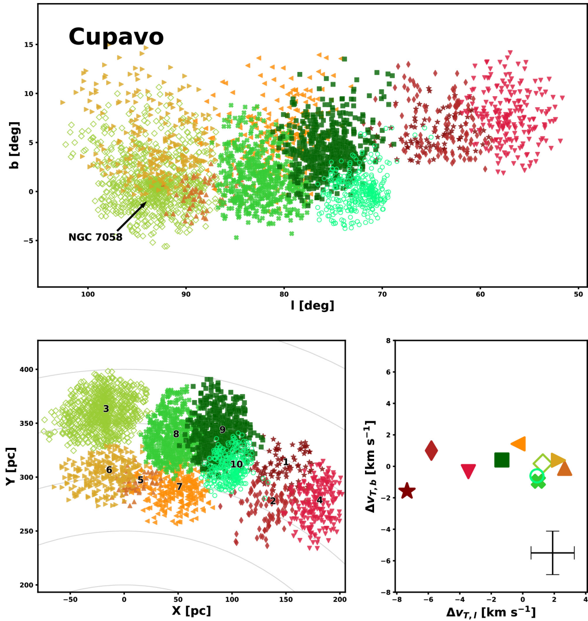
Figure 12. from Ronan Kerr et al 2024 Astrophys. J. 975 doi:10.3847/1538-4357/ad7135 https://dx.doi.org/10.3847/1538-4357/ad7135 © 2024. The Author(s). Published by the American Astronomical Society.
