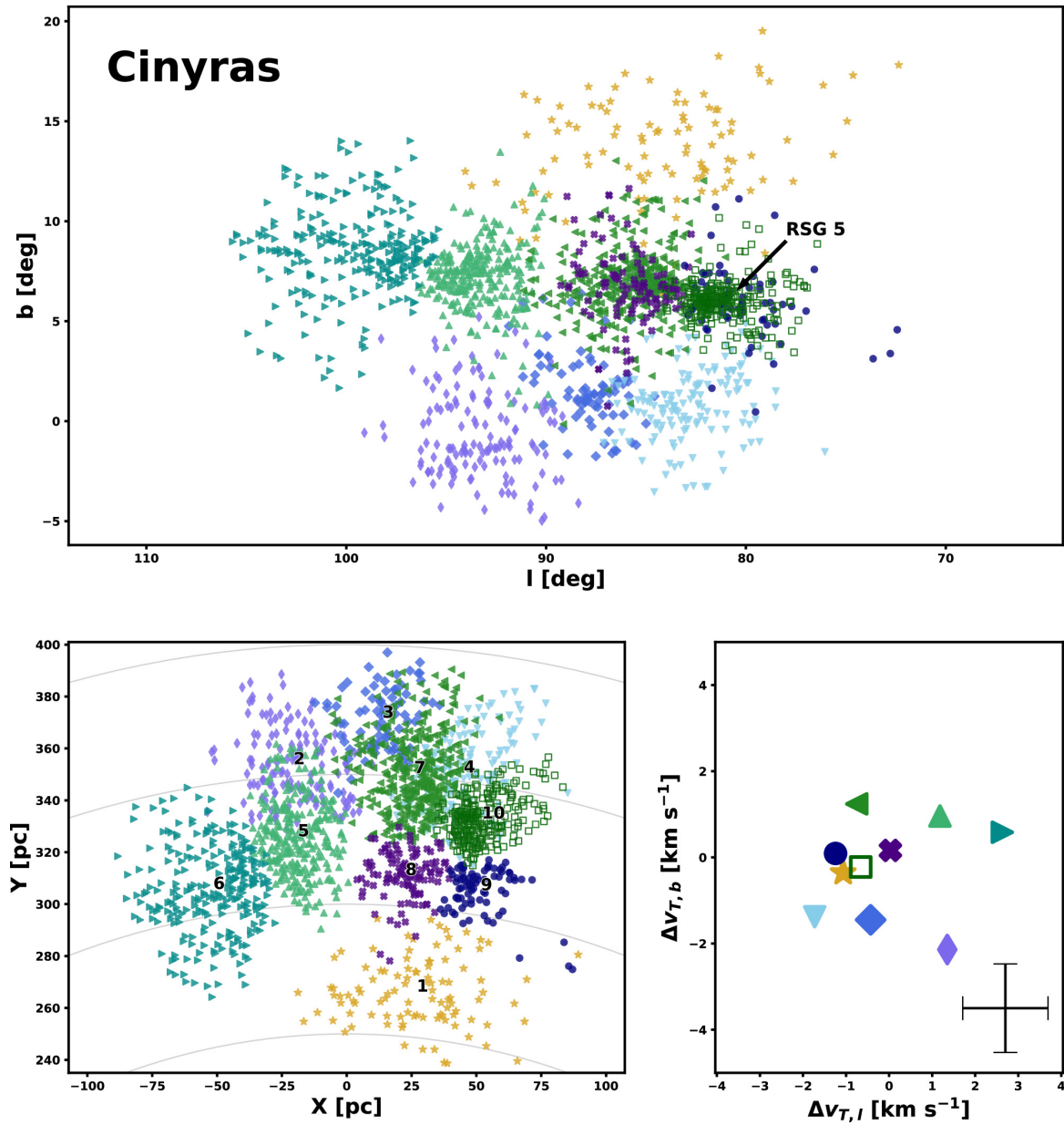
Figure 11. from Ronan Kerr et al 2024 Astrophys. J. 975 doi:10.3847/1538-4357/ad7135 https://dx.doi.org/10.3847/1538-4357/ad7135 © 2024. The Author(s). Published by the American Astronomical Society.
