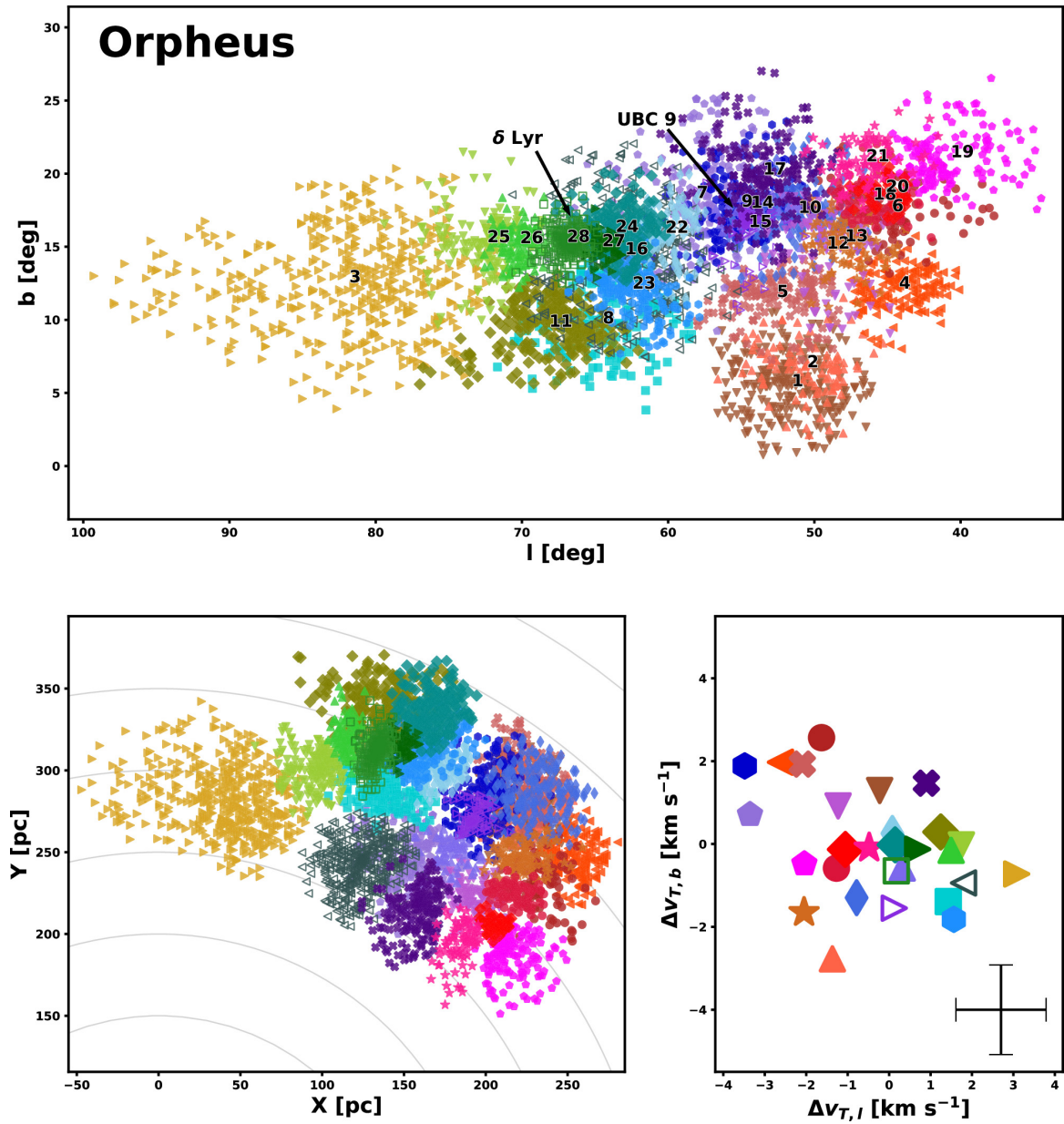
Figure 10. from Ronan Kerr et al 2024 Astrophys. J. 975 doi:10.3847/1538-4357/ad7135 https://dx.doi.org/10.3847/1538-4357/ad7135 © 2024. The Author(s). Published by the American Astronomical Society.
