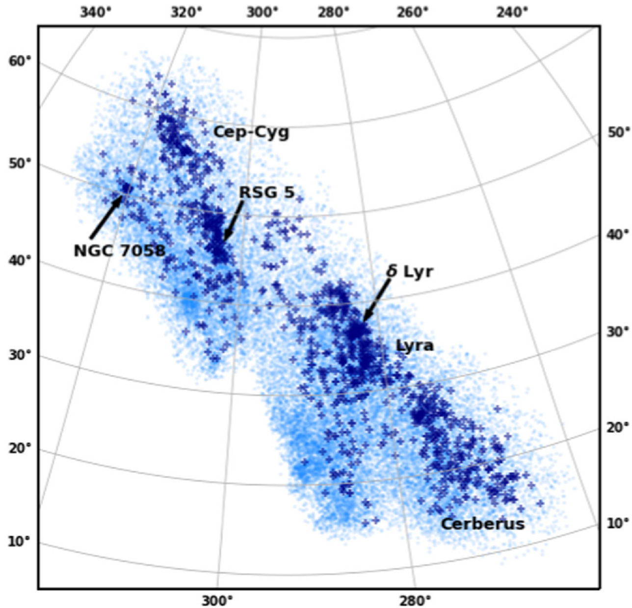
Figure 1. from Ronan Kerr et al 2024 Astrophys. J. 975 doi:10.3847/1538-4357/ad7135 https://dx.doi.org/10.3847/1538-4357/ad7135 © 2024. The Author(s). Published by the American Astronomical Society.
