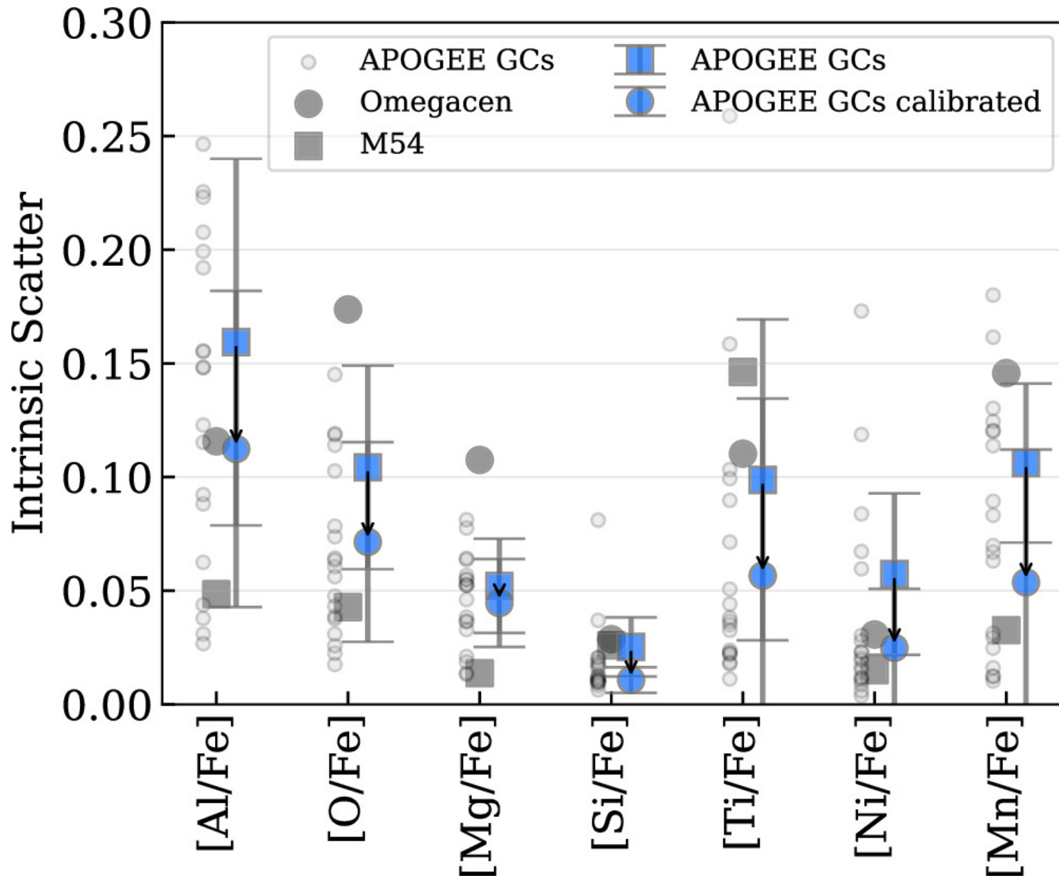
Figure 9. from Jennifer Mead et al 2024 Astrophys. J. 974 doi:10.3847/1538-4357/ad6df6 https://dx.doi.org/10.3847/1538-4357/ad6df6 © 2024. The Author(s). Published by the American Astronomical Society.
