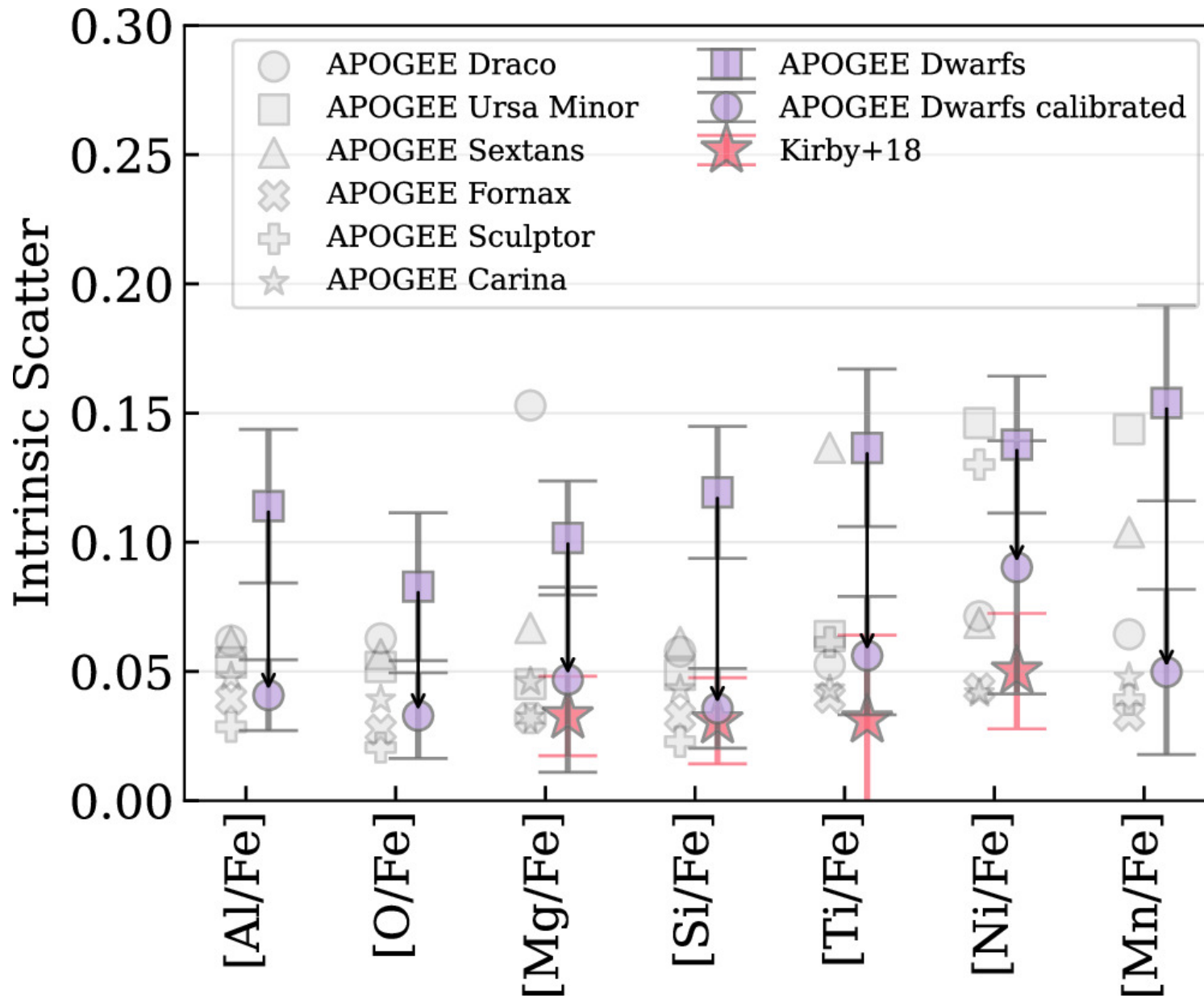
Figure 8. from Jennifer Mead et al 2024 Astrophys. J. 974 doi:10.3847/1538-4357/ad6df6 https://dx.doi.org/10.3847/1538-4357/ad6df6 © 2024. The Author(s). Published by the American Astronomical Society.
