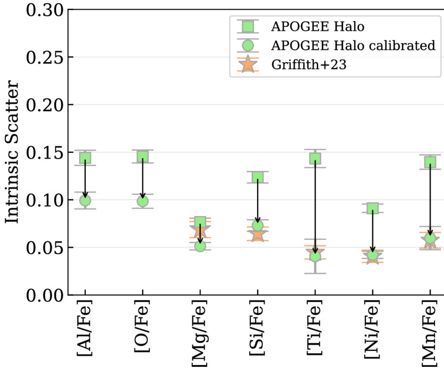
Figure 7. from Jennifer Mead et al 2024 Astrophys. J. 974 doi:10.3847/1538-4357/ad6df6 https://dx.doi.org/10.3847/1538-4357/ad6df6 © 2024. The Author(s). Published by the American Astronomical Society.
