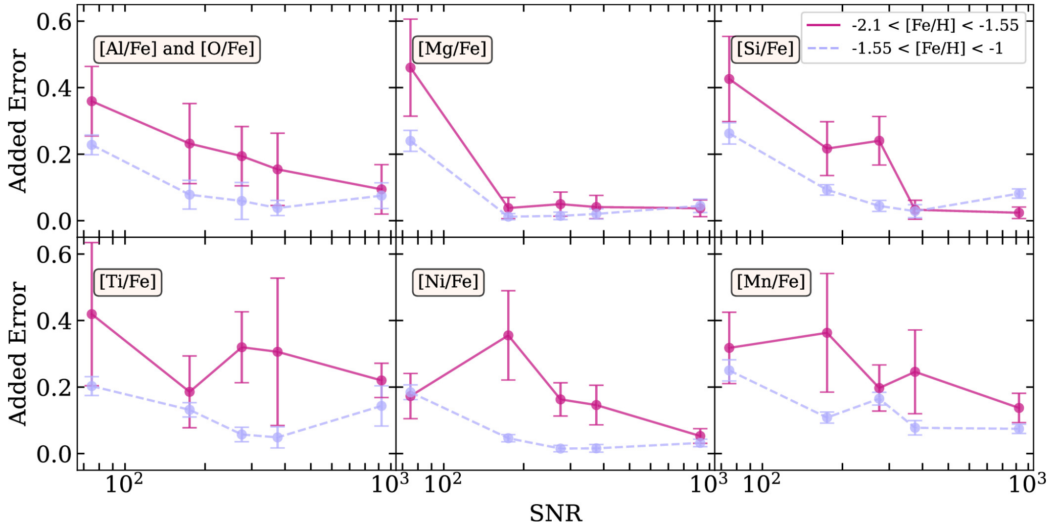
Figure 6. from Jennifer Mead et al 2024 Astrophys. J. 974 doi:10.3847/1538-4357/ad6df6 https://dx.doi.org/10.3847/1538-4357/ad6df6 © 2024. The Author(s). Published by the American Astronomical Society.
