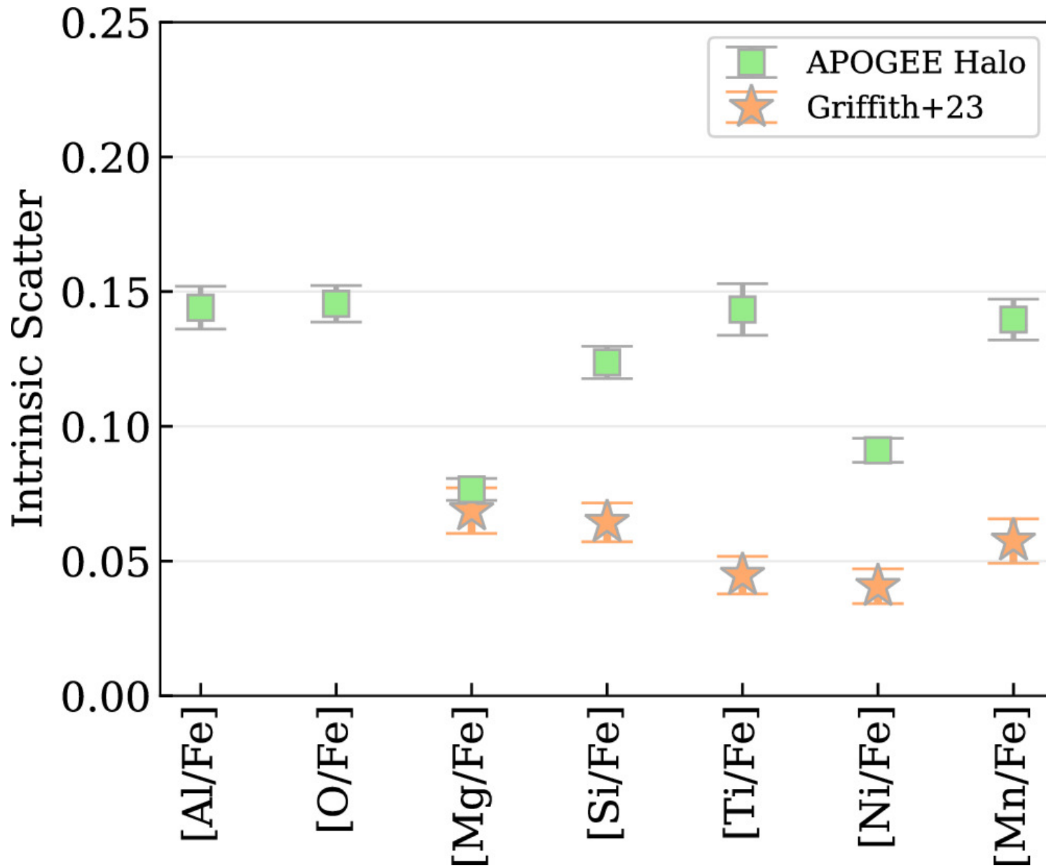
Figure 5. from Jennifer Mead et al 2024 Astrophys. J. 974 doi:10.3847/1538-4357/ad6df6 https://dx.doi.org/10.3847/1538-4357/ad6df6 © 2024. The Author(s). Published by the American Astronomical Society.
