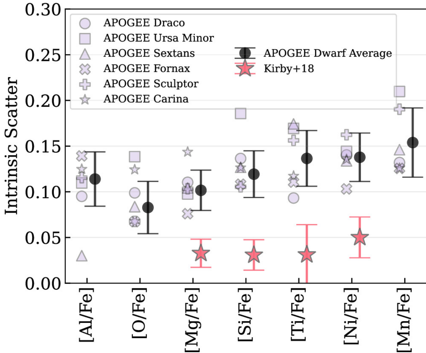
Figure 4. from Jennifer Mead et al 2024 Astrophys. J. 974 doi:10.3847/1538-4357/ad6df6 https://dx.doi.org/10.3847/1538-4357/ad6df6 © 2024. The Author(s). Published by the American Astronomical Society.
