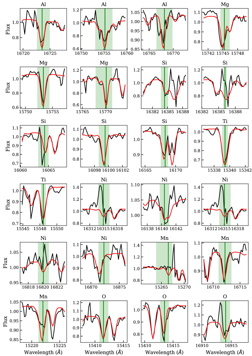
Figure 3. from Jennifer Mead et al 2024 Astrophys. J. 974 doi:10.3847/1538-4357/ad6df6 https://dx.doi.org/10.3847/1538-4357/ad6df6 © 2024. The Author(s). Published by the American Astronomical Society.
