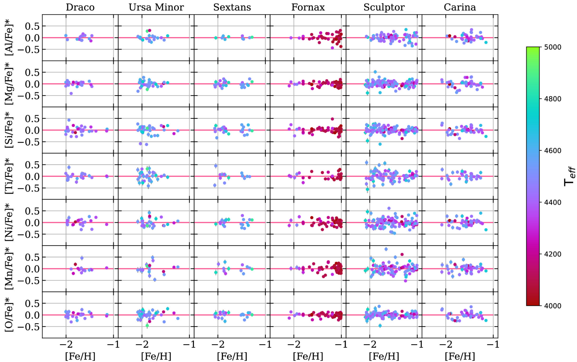
Figure 2. from Jennifer Mead et al 2024 Astrophys. J. 974 doi:10.3847/1538-4357/ad6df6 https://dx.doi.org/10.3847/1538-4357/ad6df6 © 2024. The Author(s). Published by the American Astronomical Society.
