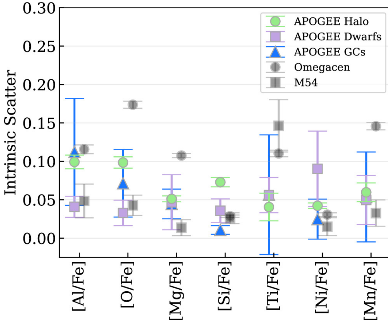
Figure 10. from Jennifer Mead et al 2024 Astrophys. J. 974 doi:10.3847/1538-4357/ad6df6 https://dx.doi.org/10.3847/1538-4357/ad6df6 © 2024. The Author(s). Published by the American Astronomical Society.
