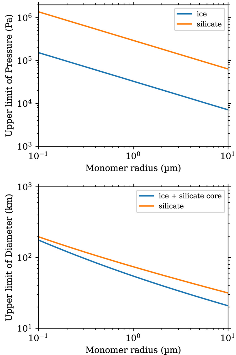
Figure 6. from Misako Tatsuuma et al 2024 Astrophys. J. 974 doi:10.3847/1538-4357/ad6a5d https://dx.doi.org/10.3847/1538-4357/ad6a5d © 2024. The Author(s). Published by the American Astronomical Society.
