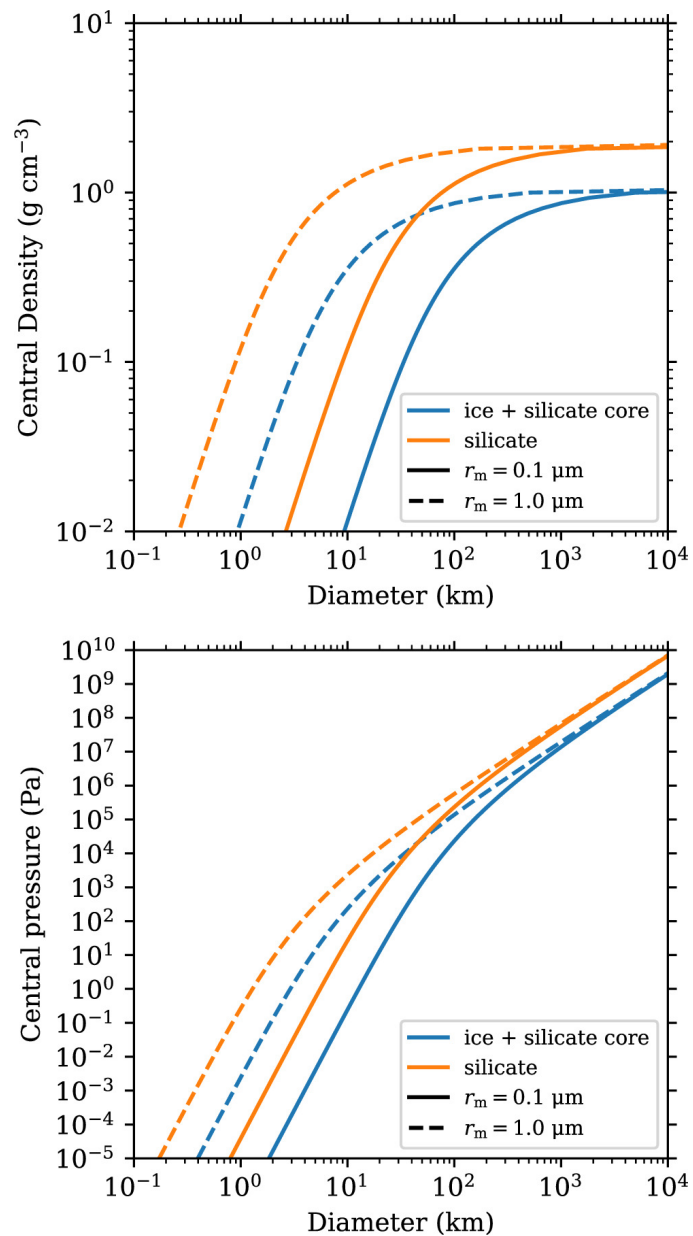
Figure 5. from Misako Tatsuuma et al 2024 Astrophys. J. 974 doi:10.3847/1538-4357/ad6a5d https://dx.doi.org/10.3847/1538-4357/ad6a5d © 2024. The Author(s). Published by the American Astronomical Society.
