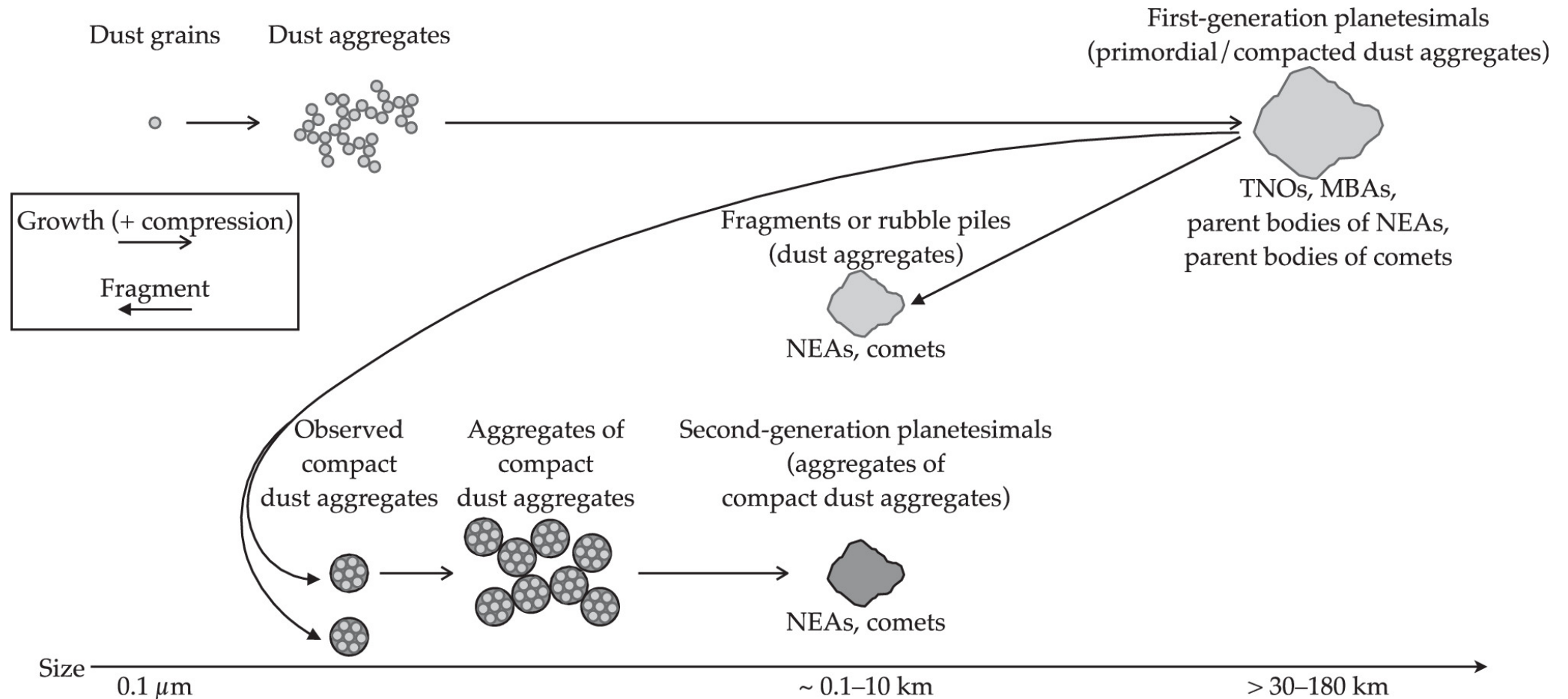
Figure 2. from Misako Tatsuuma et al 2024 Astrophys. J. 974 doi:10.3847/1538-4357/ad6a5d https://dx.doi.org/10.3847/1538-4357/ad6a5d © 2024. The Author(s). Published by the American Astronomical Society.
