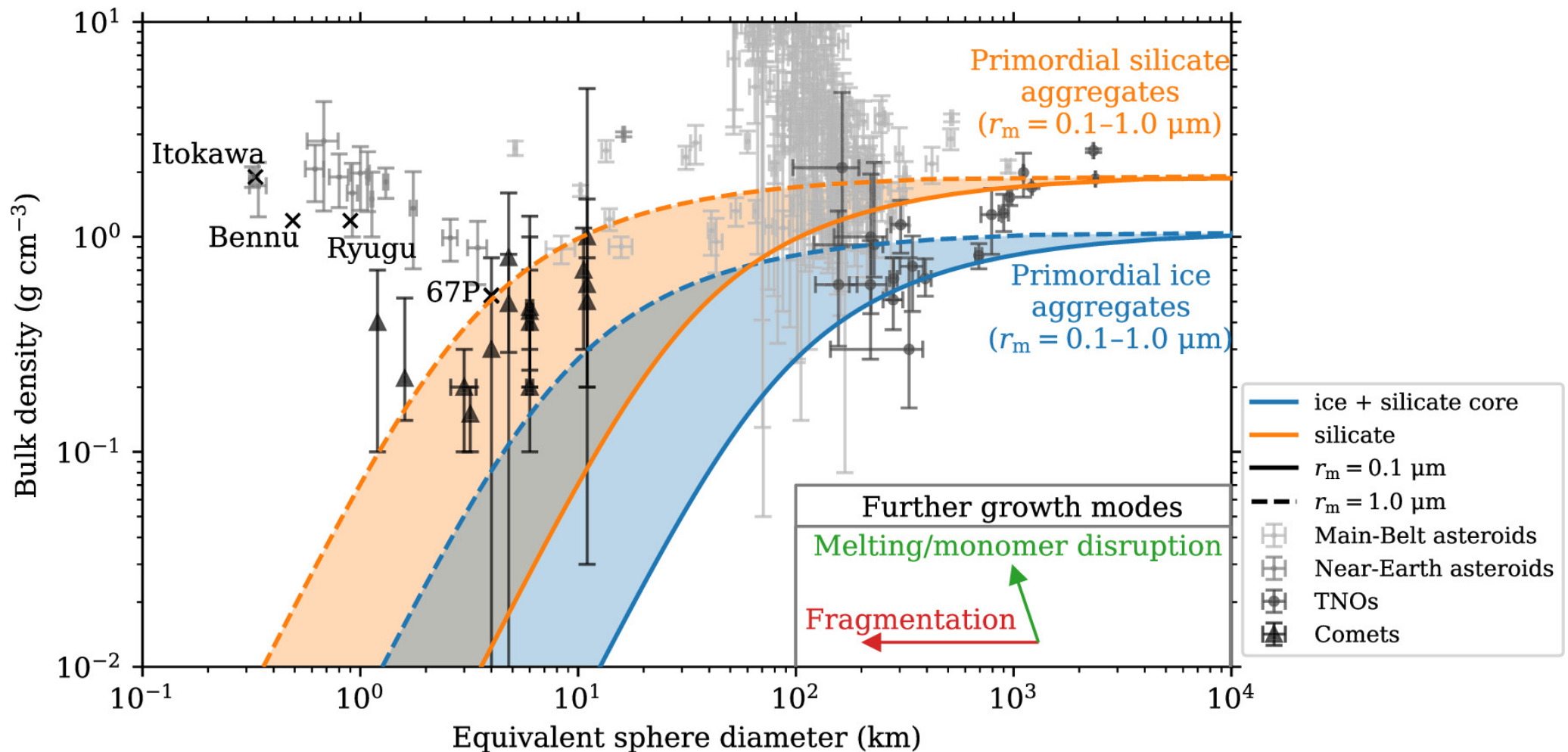
Figure 1. from Misako Tatsuuma et al 2024 Astrophys. J. 974 doi:10.3847/1538-4357/ad6a5d https://dx.doi.org/10.3847/1538-4357/ad6a5d © 2024. The Author(s). Published by the American Astronomical Society.
