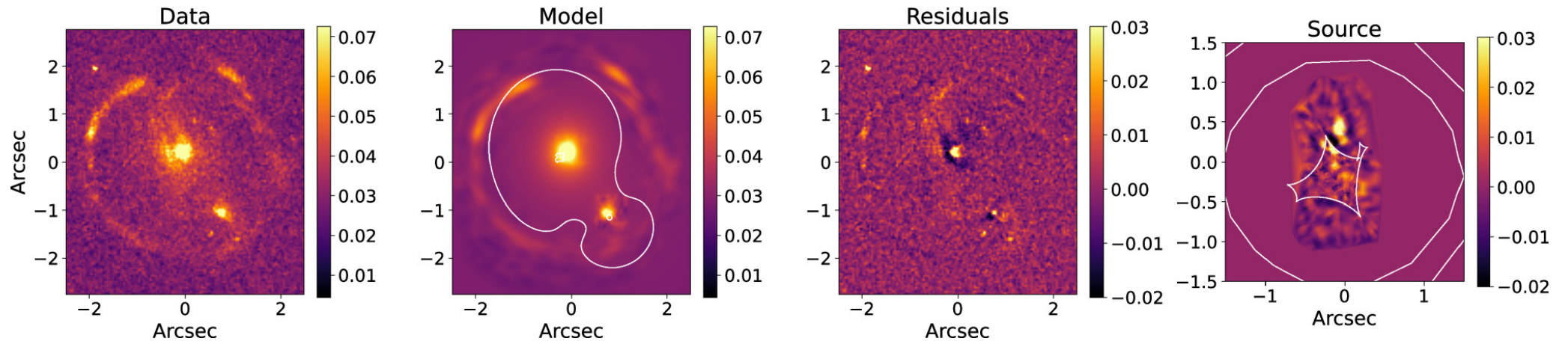
Figure 10. from Sóley Ó. Hyman et al 2024 Astrophys. J. 974 doi:10.3847/1538-4357/ad68f7 https://dx.doi.org/10.3847/1538-4357/ad68f7 © 2024. The Author(s). Published by the American Astronomical Society.
