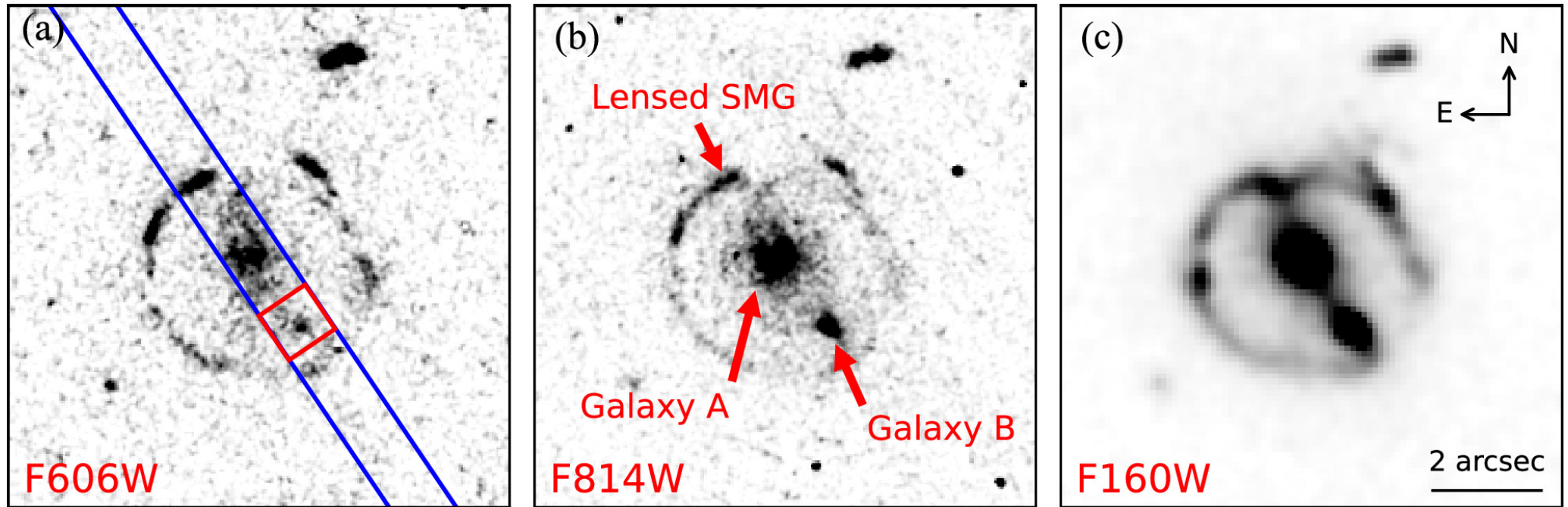
Figure 1. from Sóley Ó. Hyman et al 2024 Astrophys. J. 974 doi:10.3847/1538-4357/ad68f7 https://dx.doi.org/10.3847/1538-4357/ad68f7 © 2024. The Author(s). Published by the American Astronomical Society.
