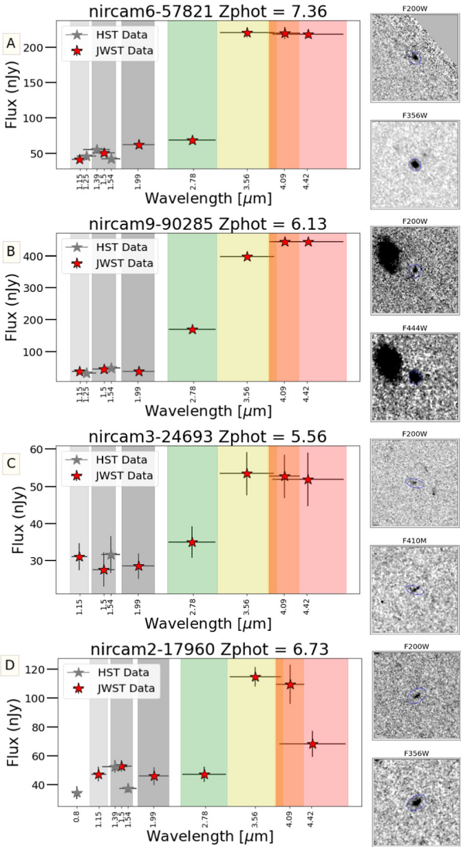
Figure 9. from Kelcey Davis et al 2024 Astrophys. J. 974 doi:10.3847/1538-4357/ad6865 https://dx.doi.org/10.3847/1538-4357/ad6865 © 2024. The Author(s). Published by the American Astronomical Society.
