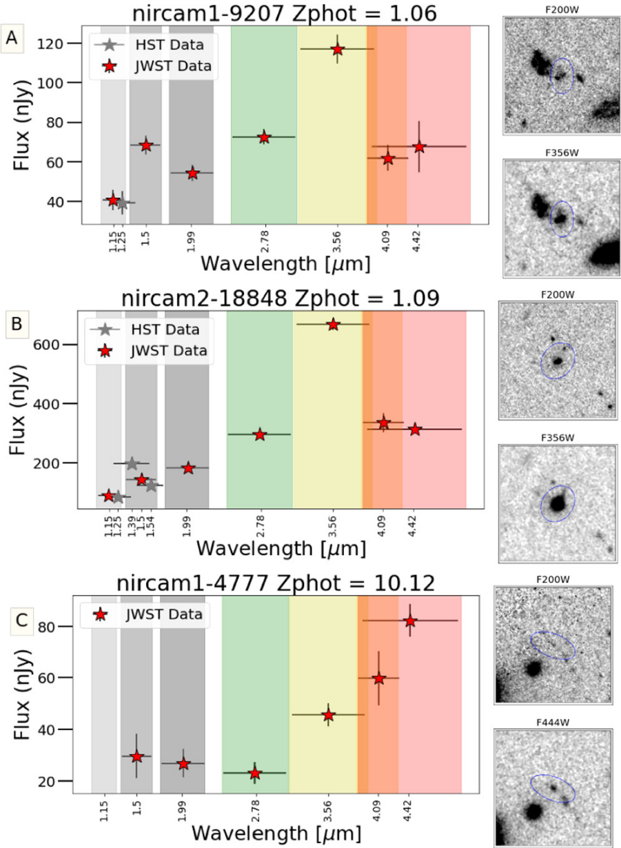
Figure 8. from Kelcey Davis et al 2024 Astrophys. J. 974 doi:10.3847/1538-4357/ad6865 https://dx.doi.org/10.3847/1538-4357/ad6865 © 2024. The Author(s). Published by the American Astronomical Society.
