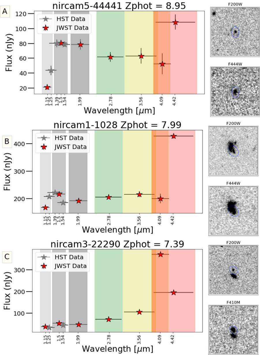
Figure 6. from Kelcey Davis et al 2024 Astrophys. J. 974 doi:10.3847/1538-4357/ad6865 https://dx.doi.org/10.3847/1538-4357/ad6865 © 2024. The Author(s). Published by the American Astronomical Society.
