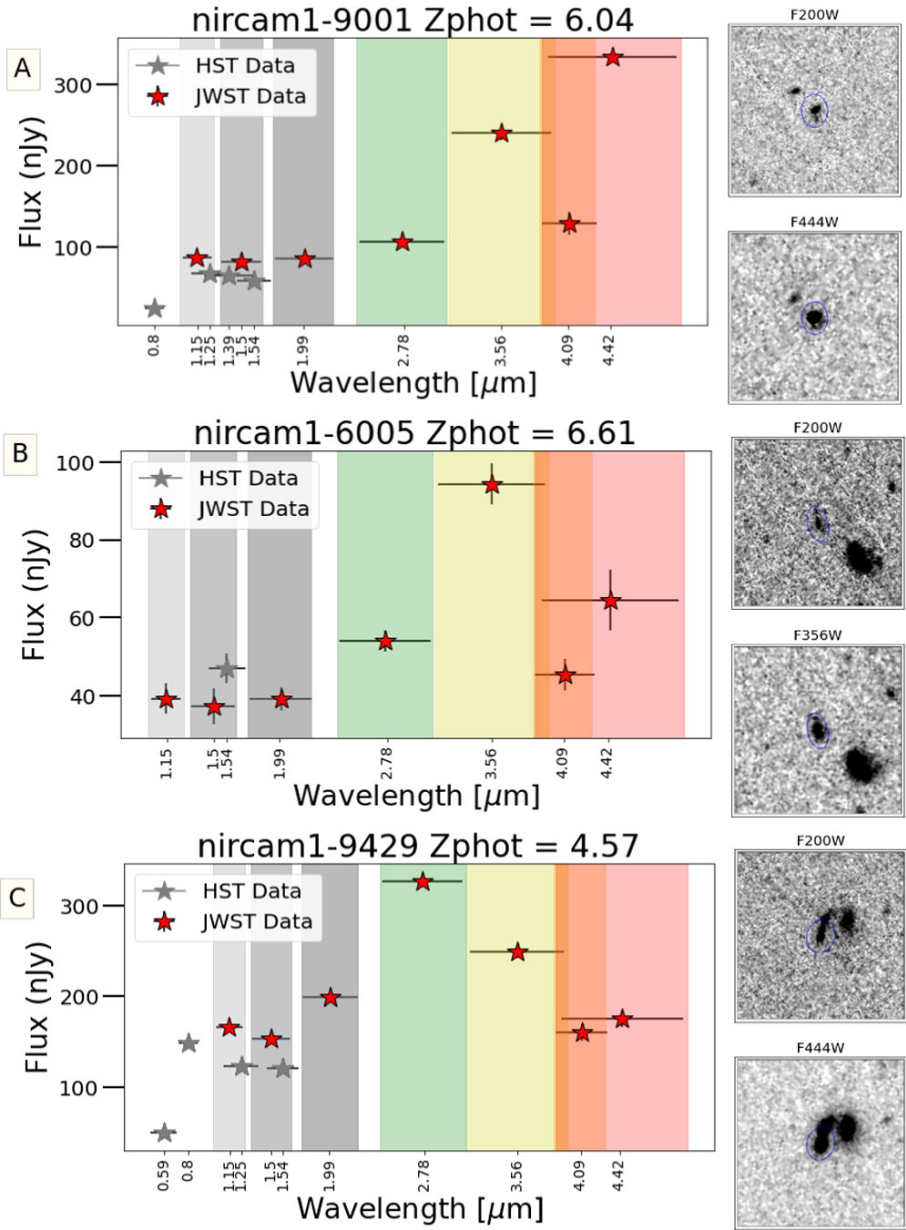
Figure 5. from Kelcey Davis et al 2024 Astrophys. J. 974 doi:10.3847/1538-4357/ad6865 https://dx.doi.org/10.3847/1538-4357/ad6865 © 2024. The Author(s). Published by the American Astronomical Society.
