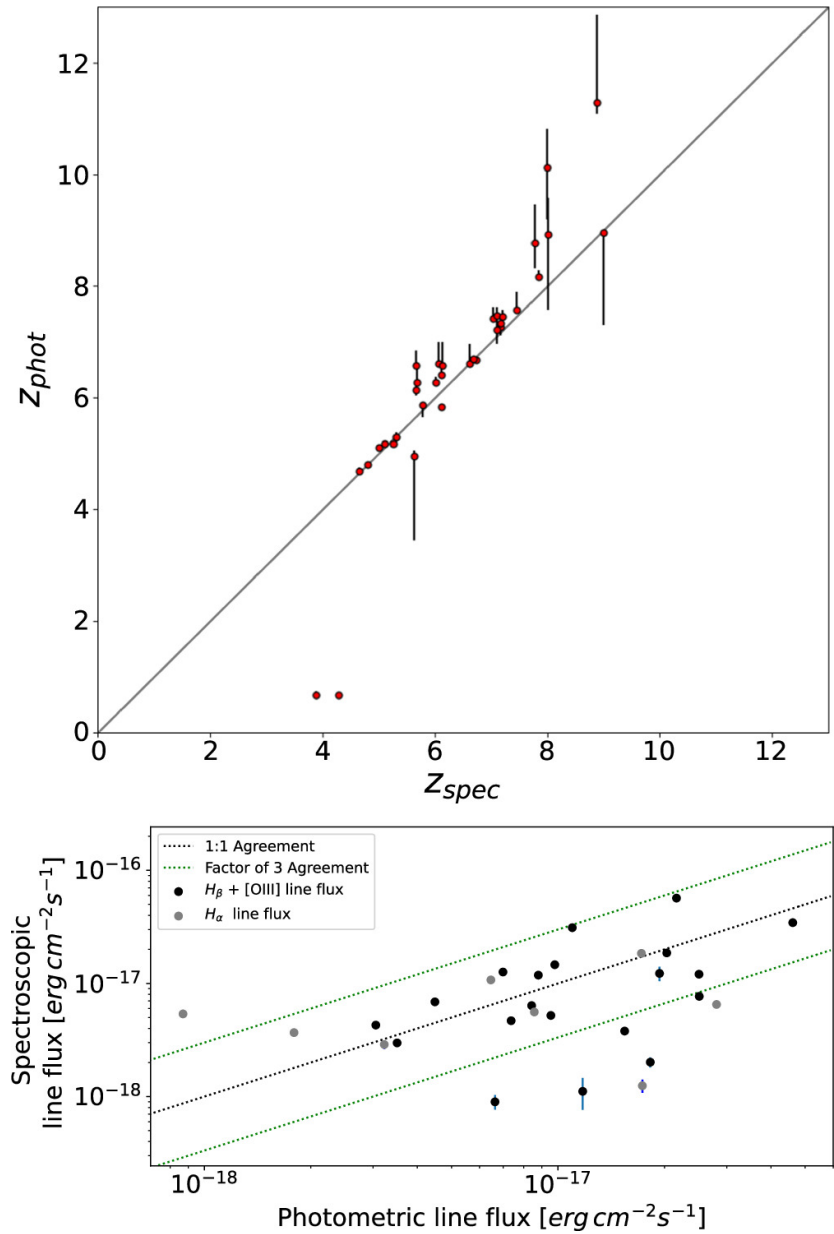
Figure 4. from Kelcey Davis et al 2024 Astrophys. J. 974 doi:10.3847/1538-4357/ad6865 https://dx.doi.org/10.3847/1538-4357/ad6865 © 2024. The Author(s). Published by the American Astronomical Society.
