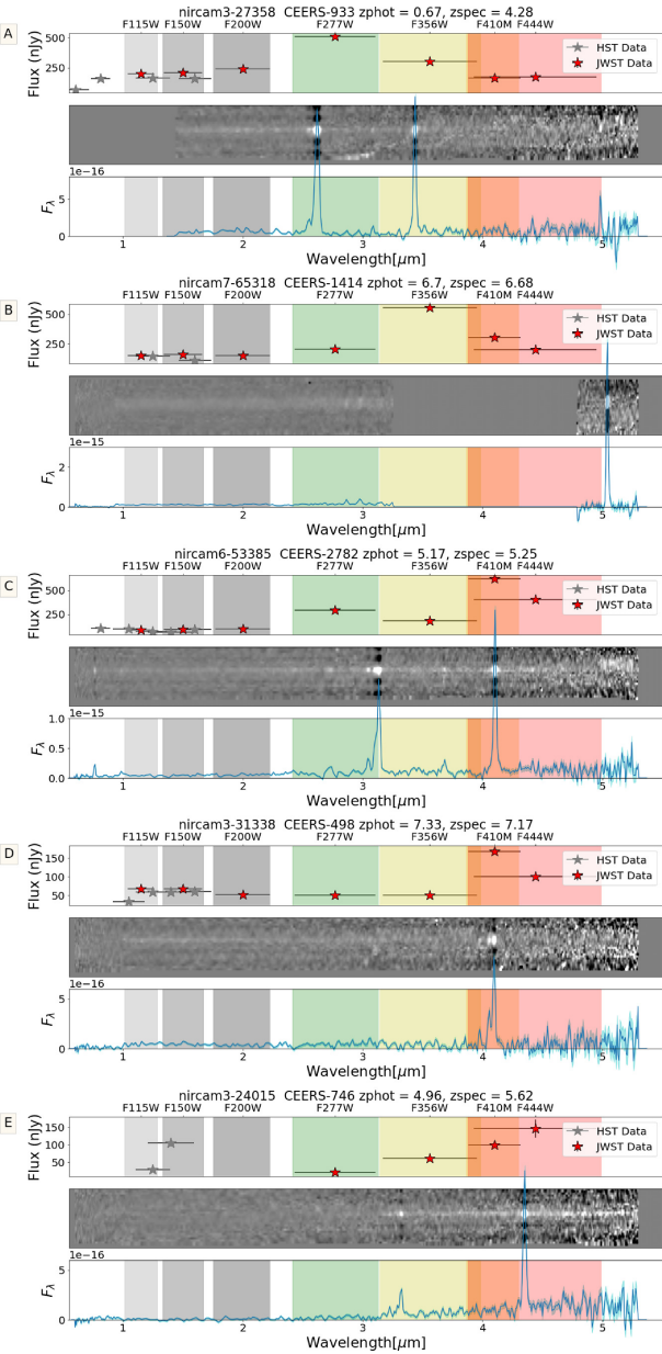
Figure 3. from Kelcey Davis et al 2024 Astrophys. J. 974 doi:10.3847/1538-4357/ad6865 https://dx.doi.org/10.3847/1538-4357/ad6865 © 2024. The Author(s). Published by the American Astronomical Society.
