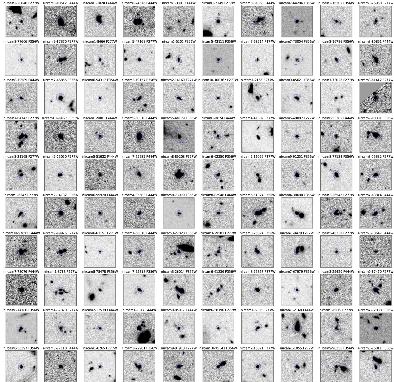
Figure 20. from Kelcey Davis et al 2024 Astrophys. J. 974 doi:10.3847/1538-4357/ad6865 https://dx.doi.org/10.3847/1538-4357/ad6865 © 2024. The Author(s). Published by the American Astronomical Society.
