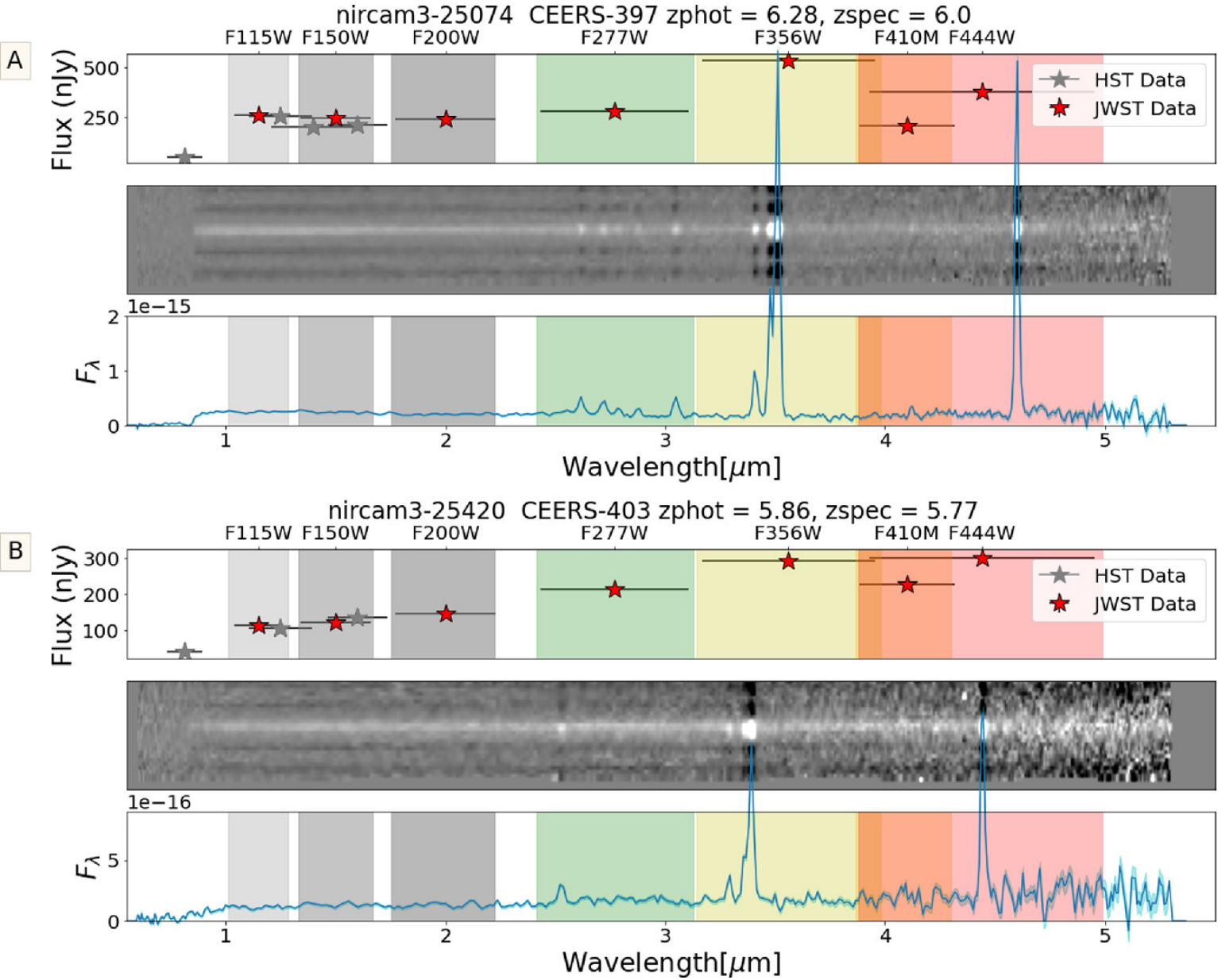
Figure 2. from Kelcey Davis et al 2024 Astrophys. J. 974 doi:10.3847/1538-4357/ad6865 https://dx.doi.org/10.3847/1538-4357/ad6865 © 2024. The Author(s). Published by the American Astronomical Society.
