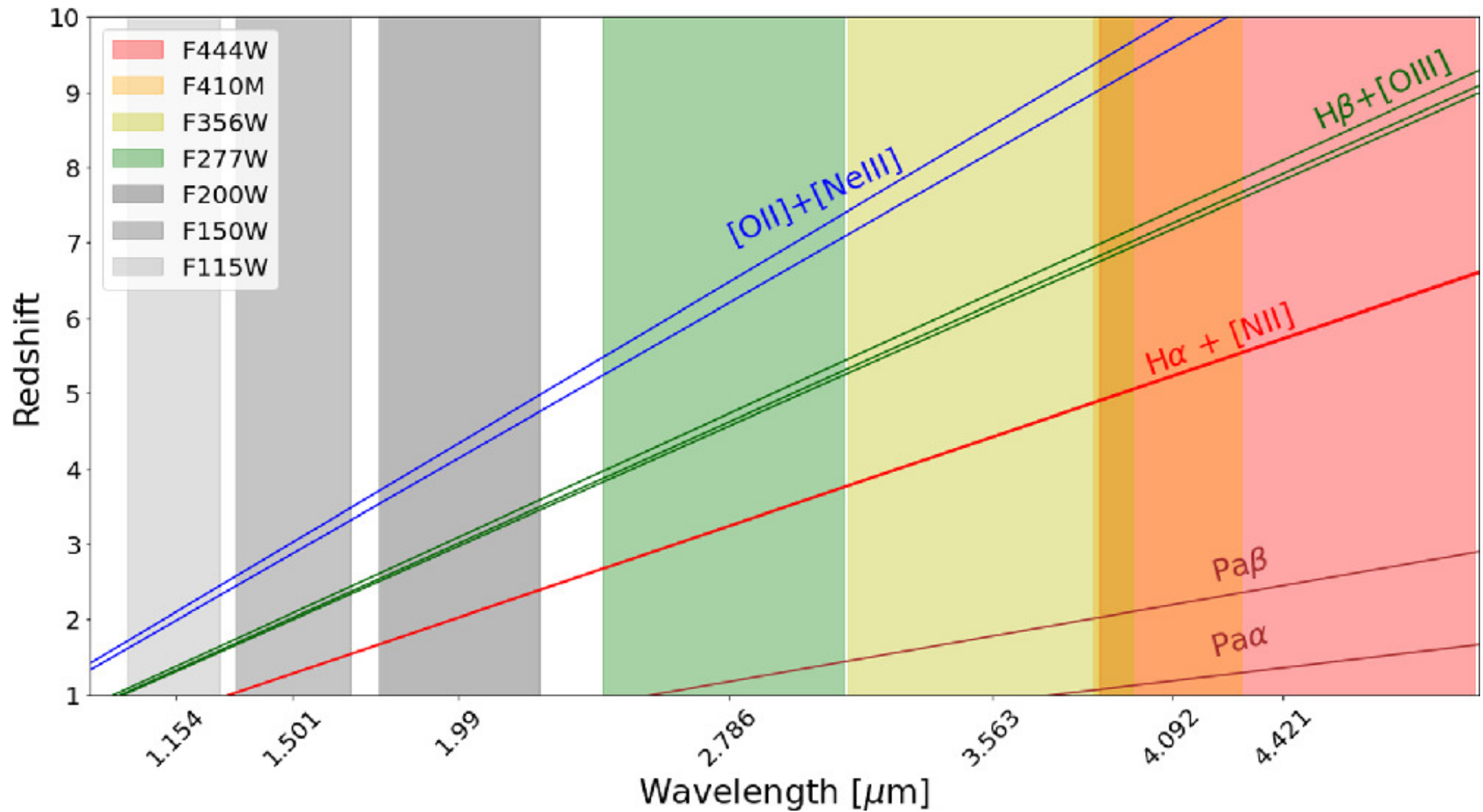
Figure 1. from Kelcey Davis et al 2024 Astrophys. J. 974 doi:10.3847/1538-4357/ad6865 https://dx.doi.org/10.3847/1538-4357/ad6865 © 2024. The Author(s). Published by the American Astronomical Society.
