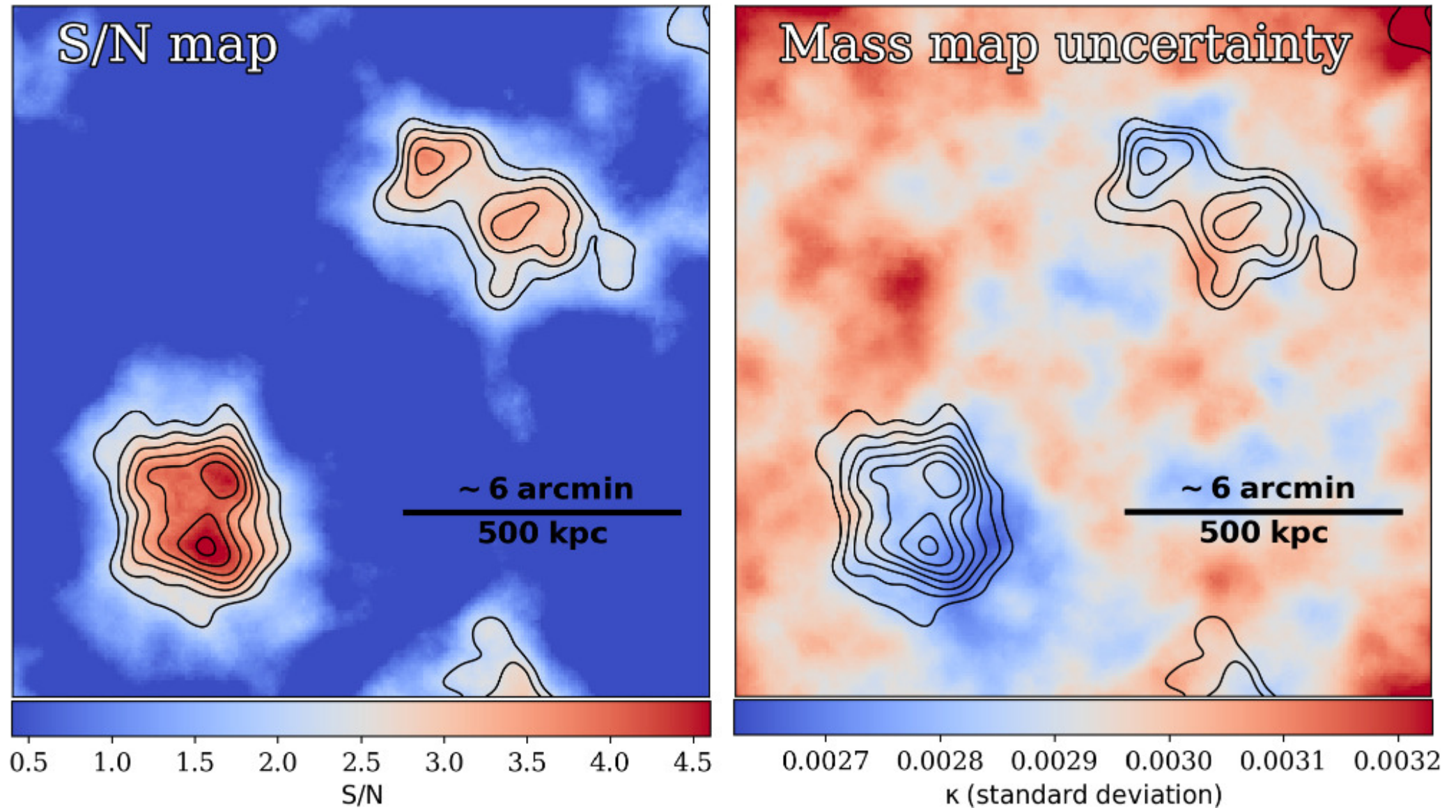
Figure 8. from Eunmo Ahn et al 2024 Astrophys. J. 973 doi:10.3847/1538-4357/ad65dc https://dx.doi.org/10.3847/1538-4357/ad65dc © 2024. The Author(s). Published by the American Astronomical Society.
