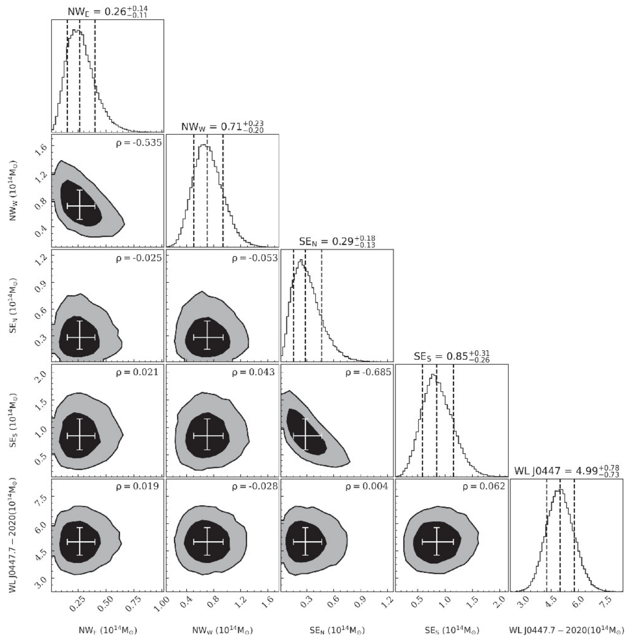
Figure 7. from Eunmo Ahn et al 2024 Astrophys. J. 973 doi:10.3847/1538-4357/ad65dc https://dx.doi.org/10.3847/1538-4357/ad65dc © 2024. The Author(s). Published by the American Astronomical Society.
