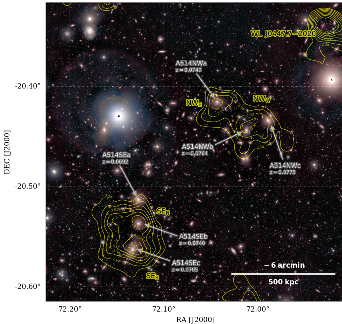
Figure 4. from Eunmo Ahn et al 2024 Astrophys. J. 973 doi:10.3847/1538-4357/ad65dc https://dx.doi.org/10.3847/1538-4357/ad65dc © 2024. The Author(s). Published by the American Astronomical Society.
